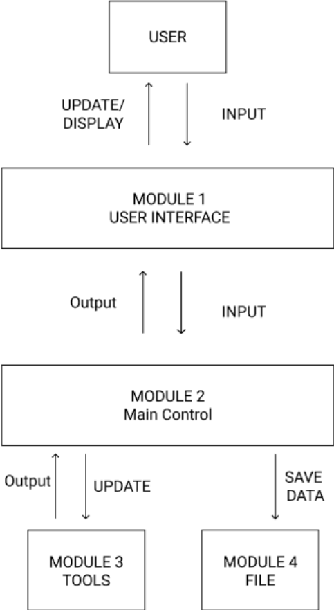
Figure 4-2. Level 1 DFD
