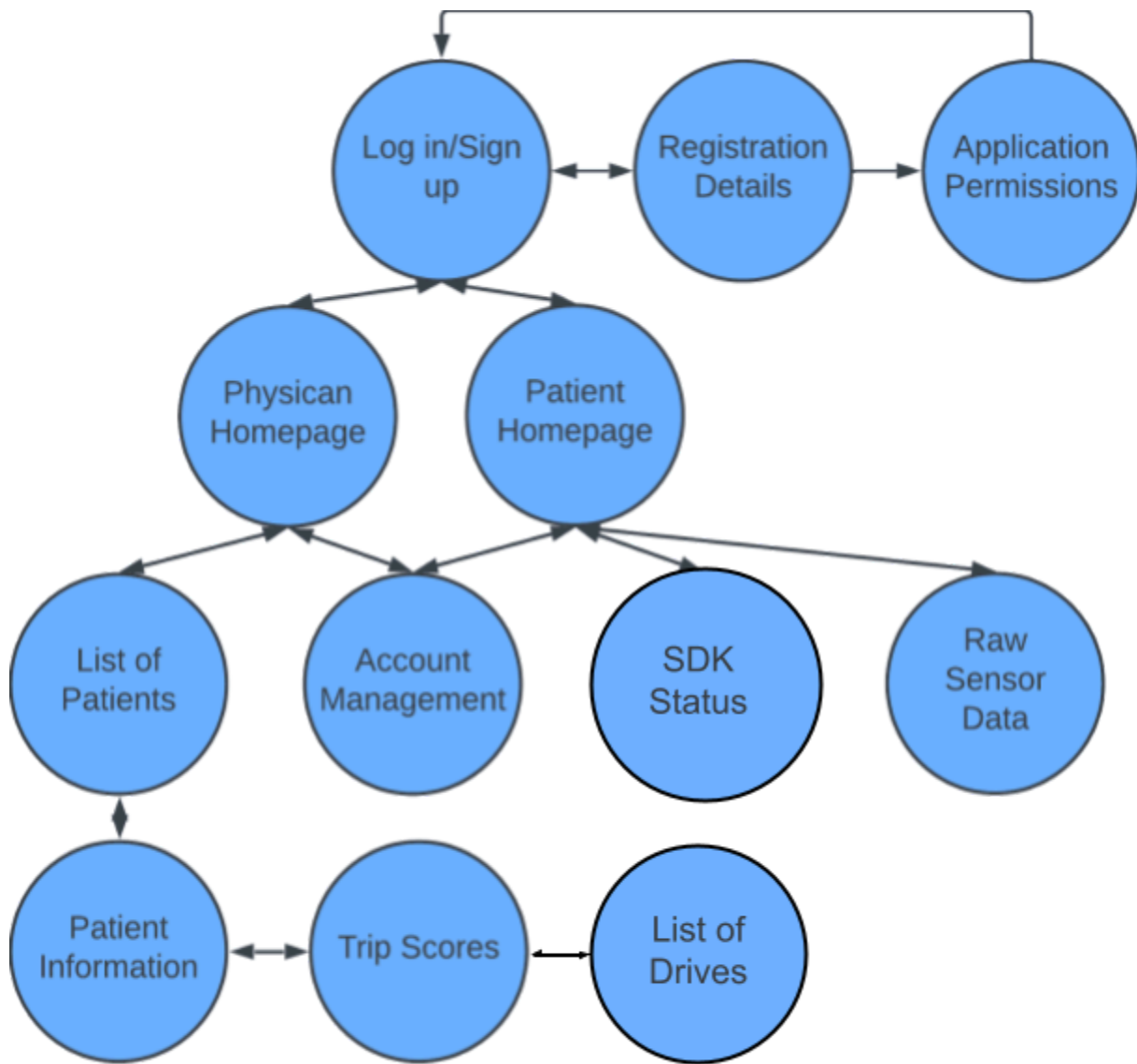
Entity-Relationship Diagram
