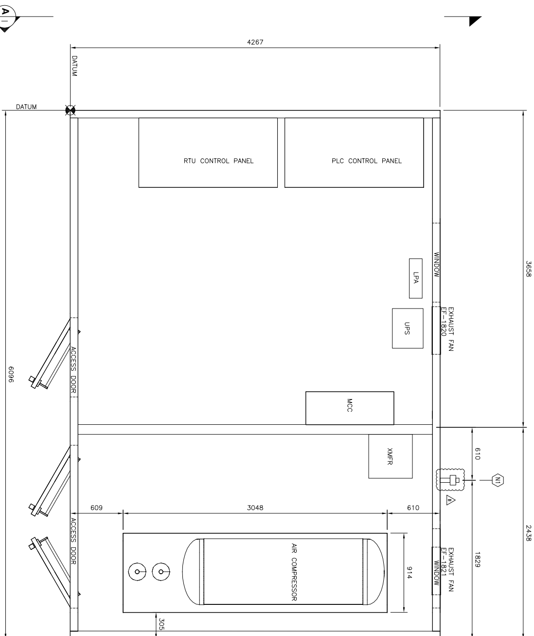
MCC/AIR COMPRESSOR BUILDING BU-1820 PLAN VIEW
