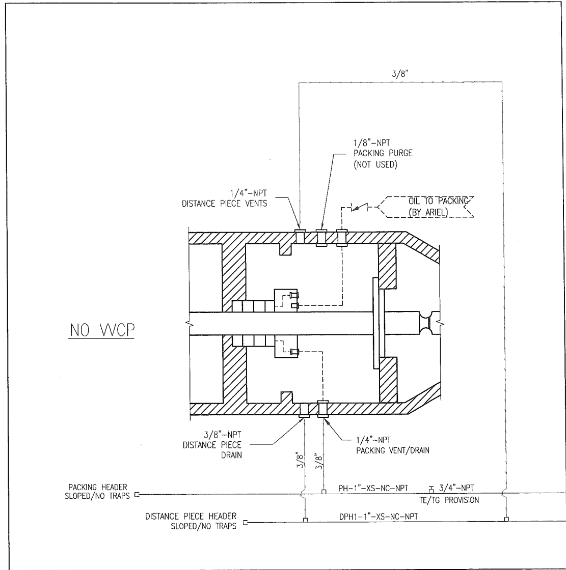
DISTANCE PIECE / PACKING VENT & DRAIN STANDARD COMPARTMENT, R:J CLASS (TYP EACH CYLINDER)
