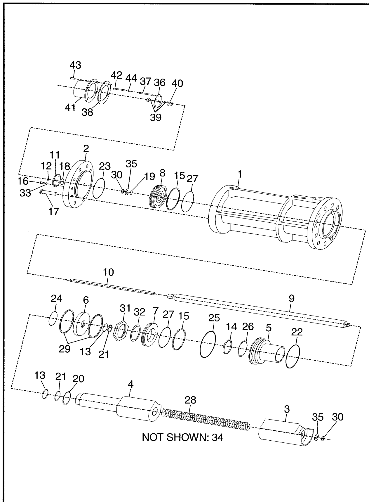
Figure 2. Slide Valve/Stop Assembly, 163.
