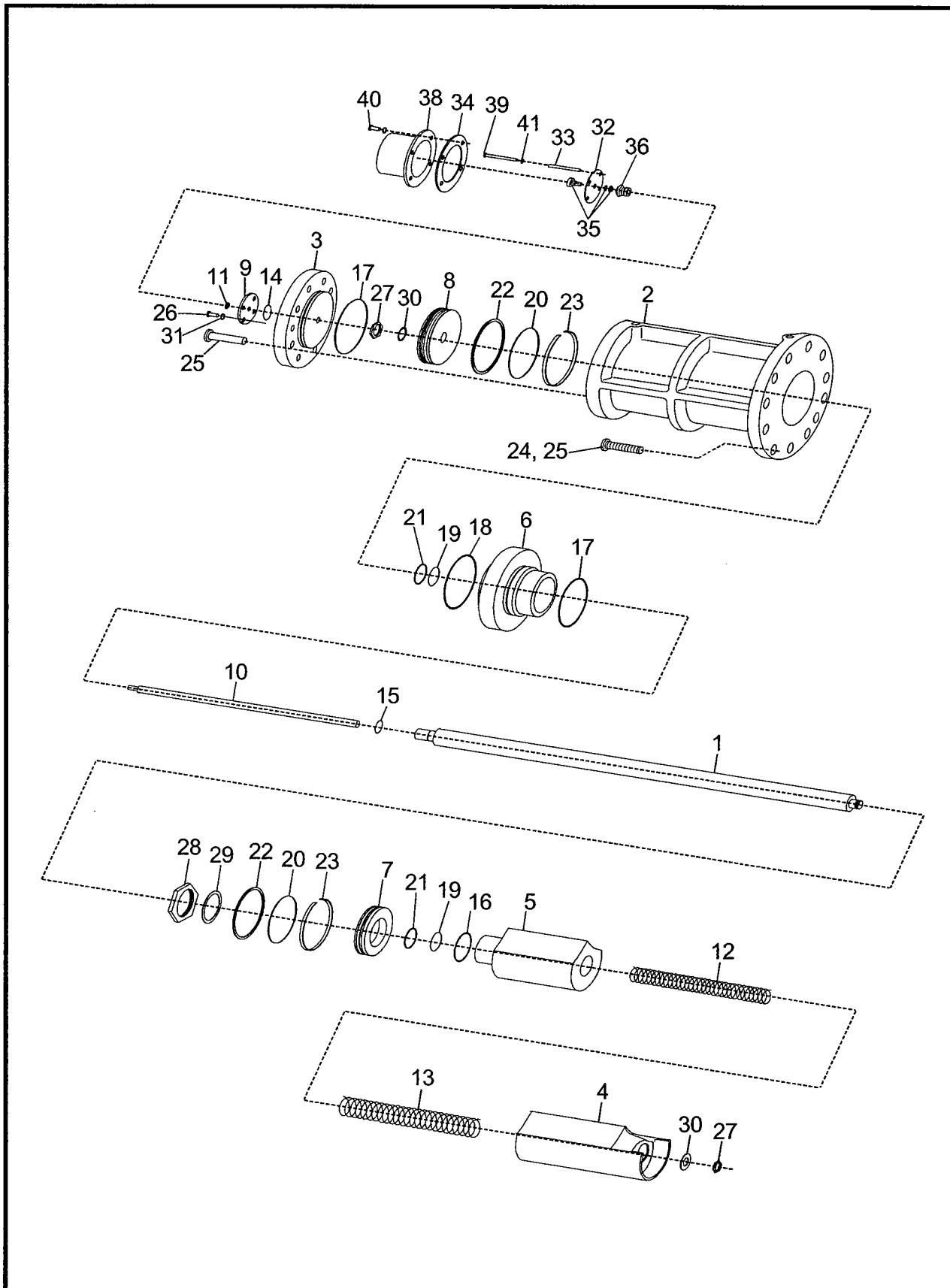
Figure 15. Slide Valve/Stop Assembly, 355.
