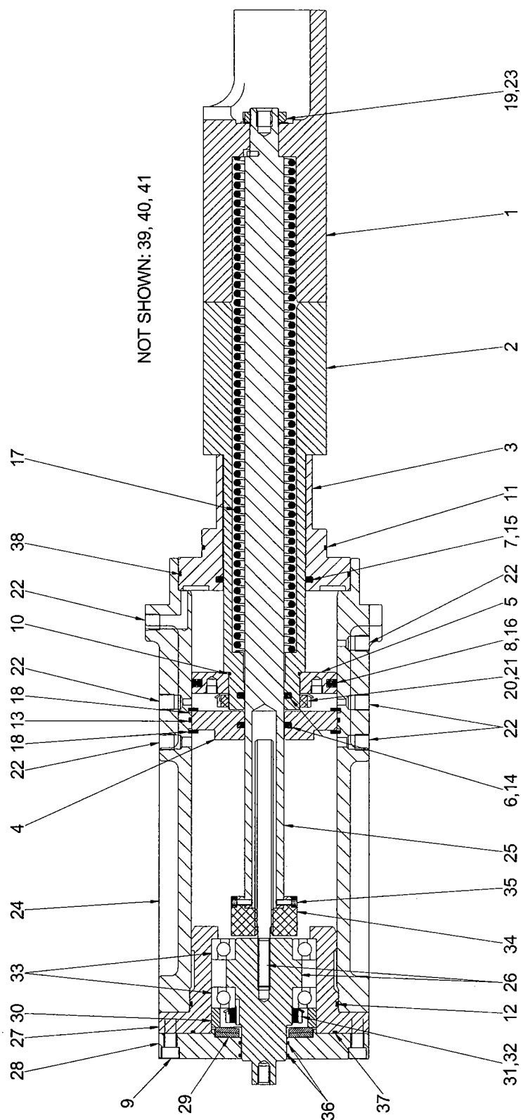
Figure 6. Slide Valve/Stop Assembly, Handwheel, 193.
