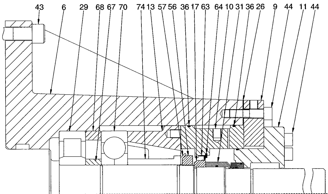
SIDE VIEW SHAFT SEAL ASSEMBLY
