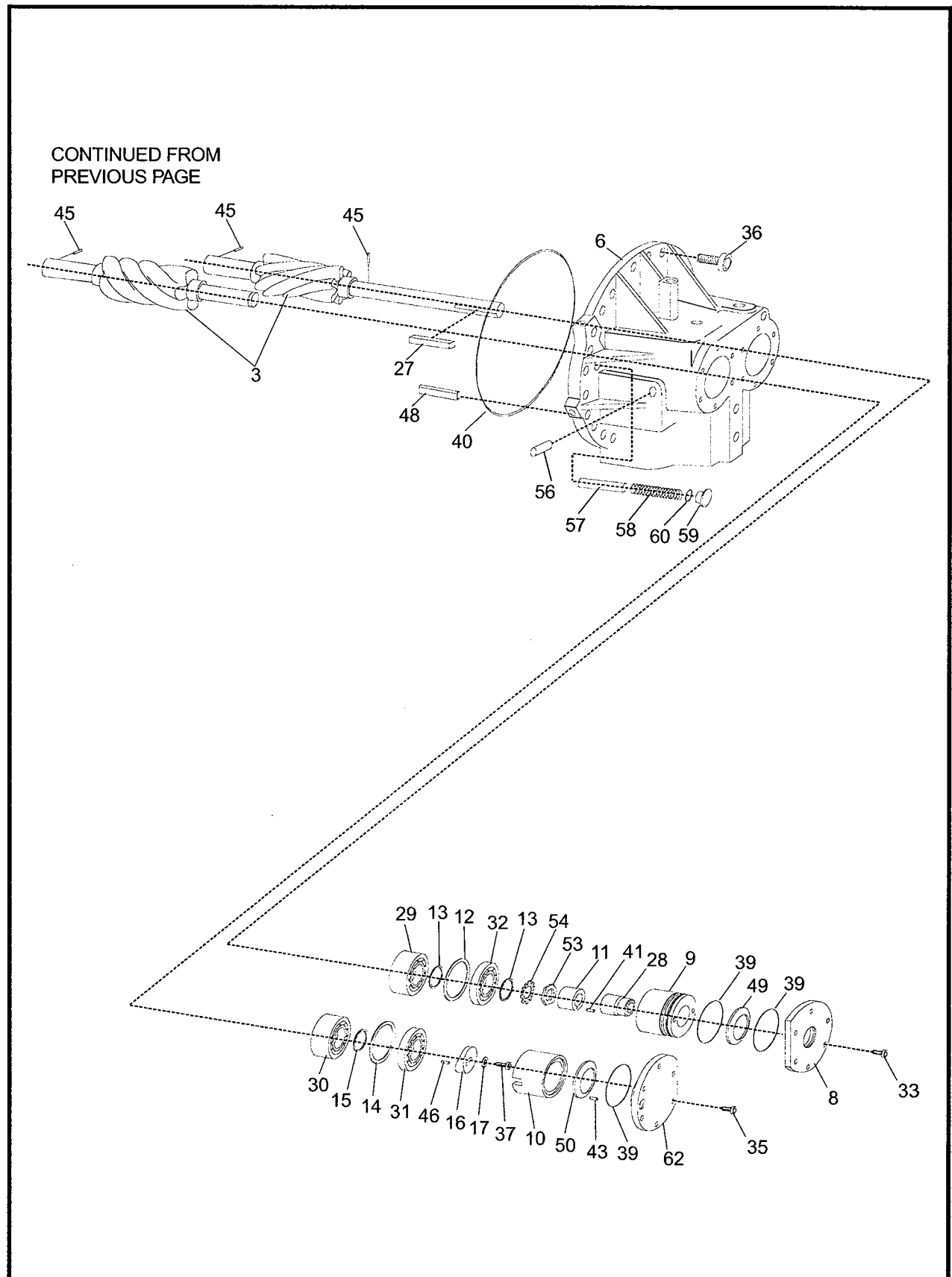
Figure 4b. Screw Compressor, 193.
