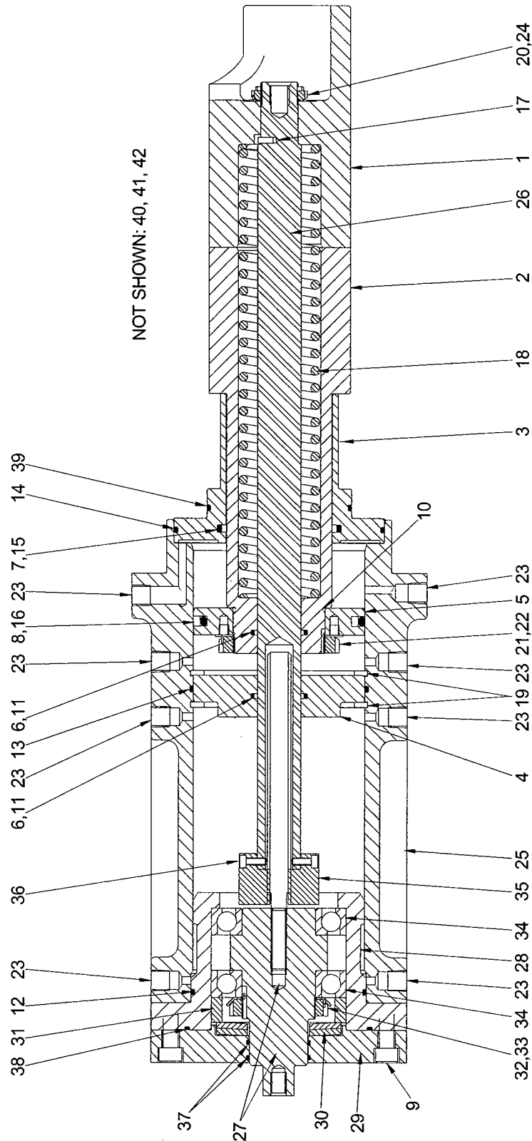
Figure 3. Slide Valve/Stop Assembly, Handwheel, 163
