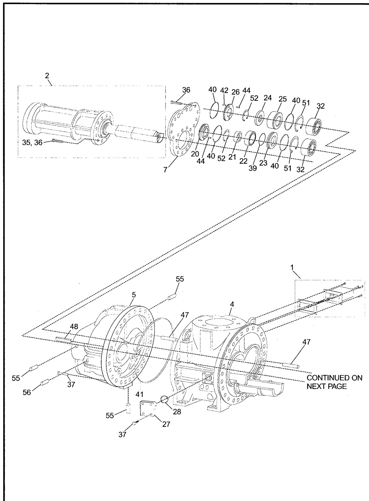
Figure 1a. Screw Compressor, 163.
