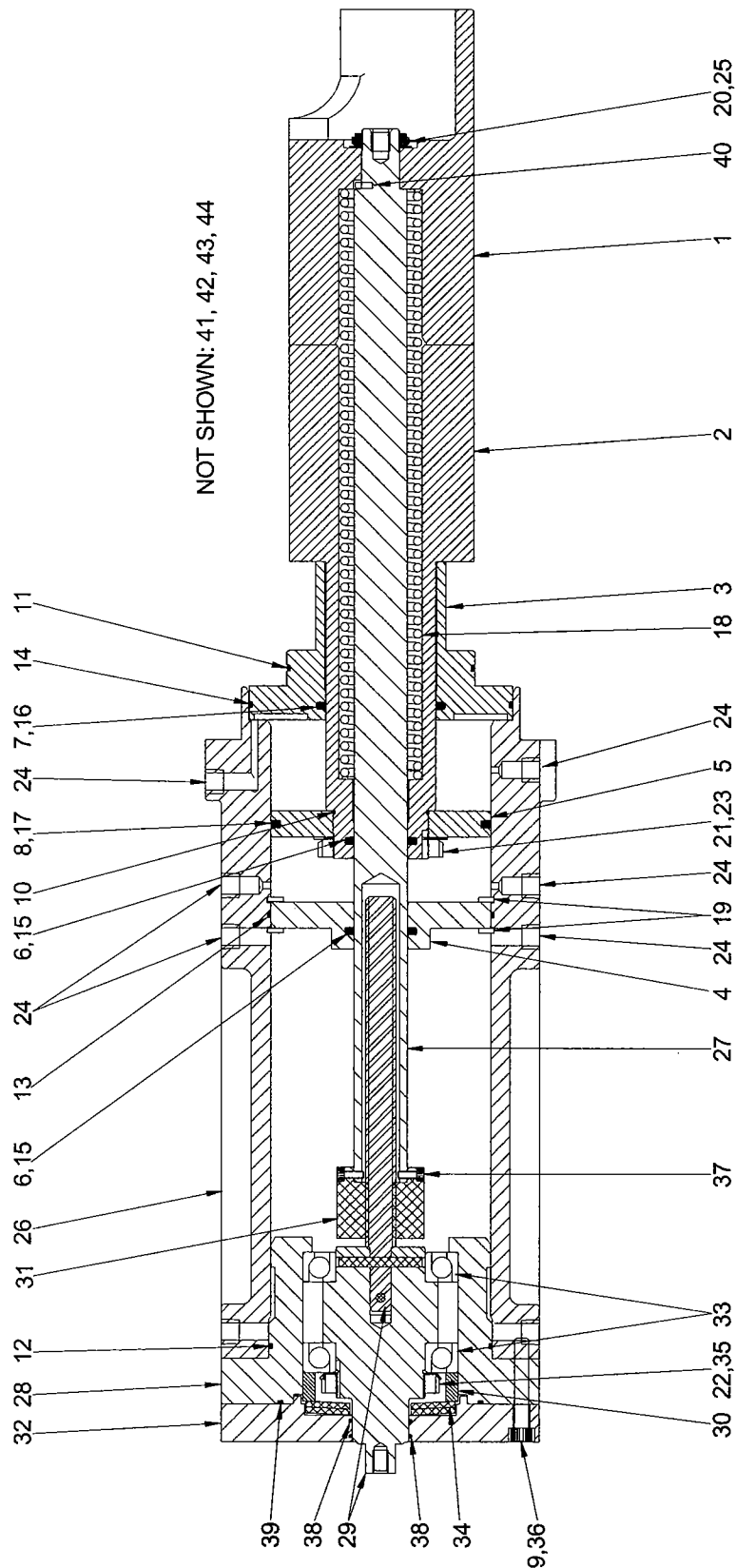
Figure 9. Slide Valve/Stop, Handwheel, 233.
