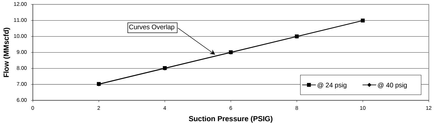
FLOW CURVE (flow rates guaranteed to +/- 5%)
