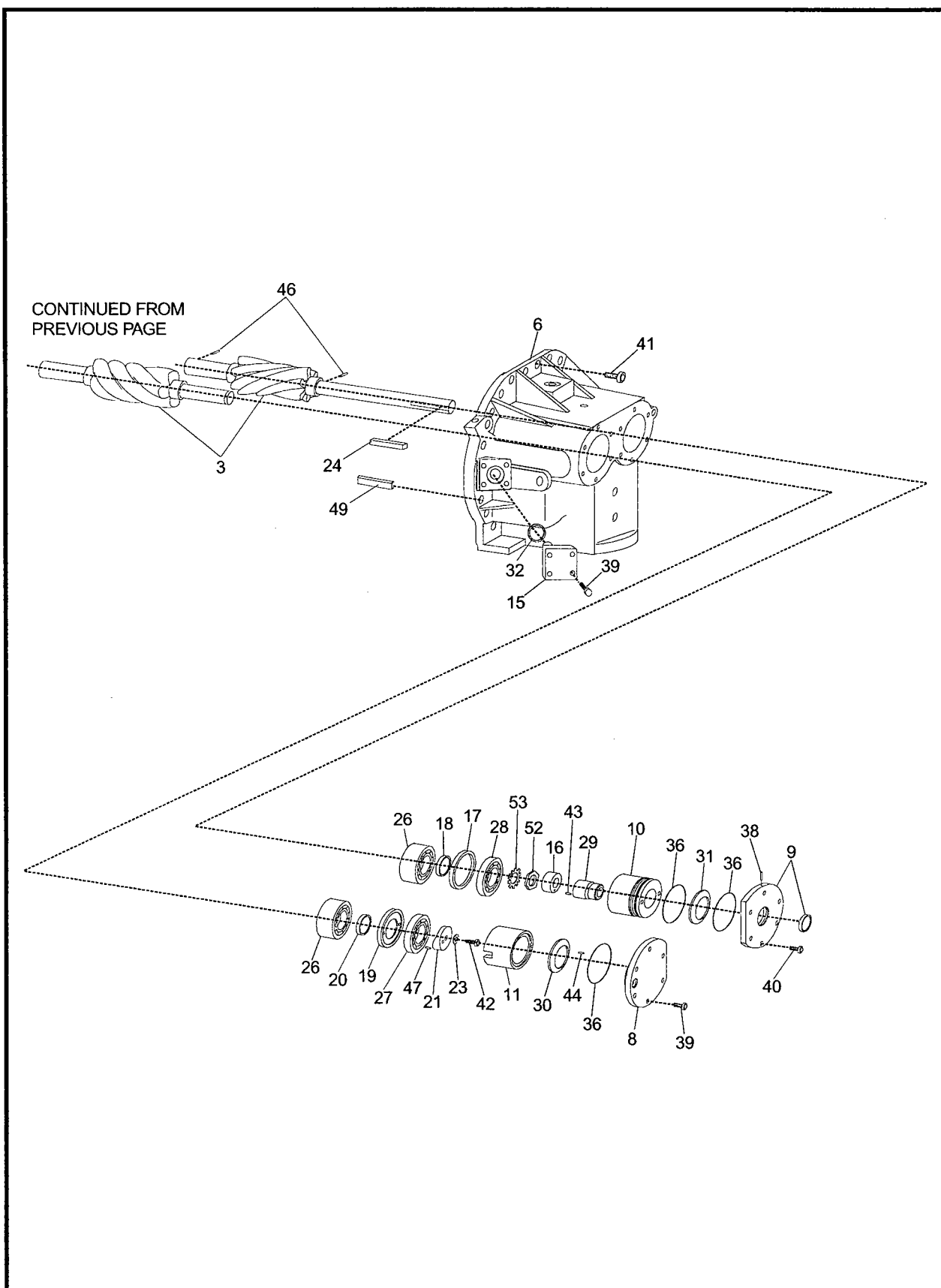
Figure 10b. Screw Compressor, 283.
