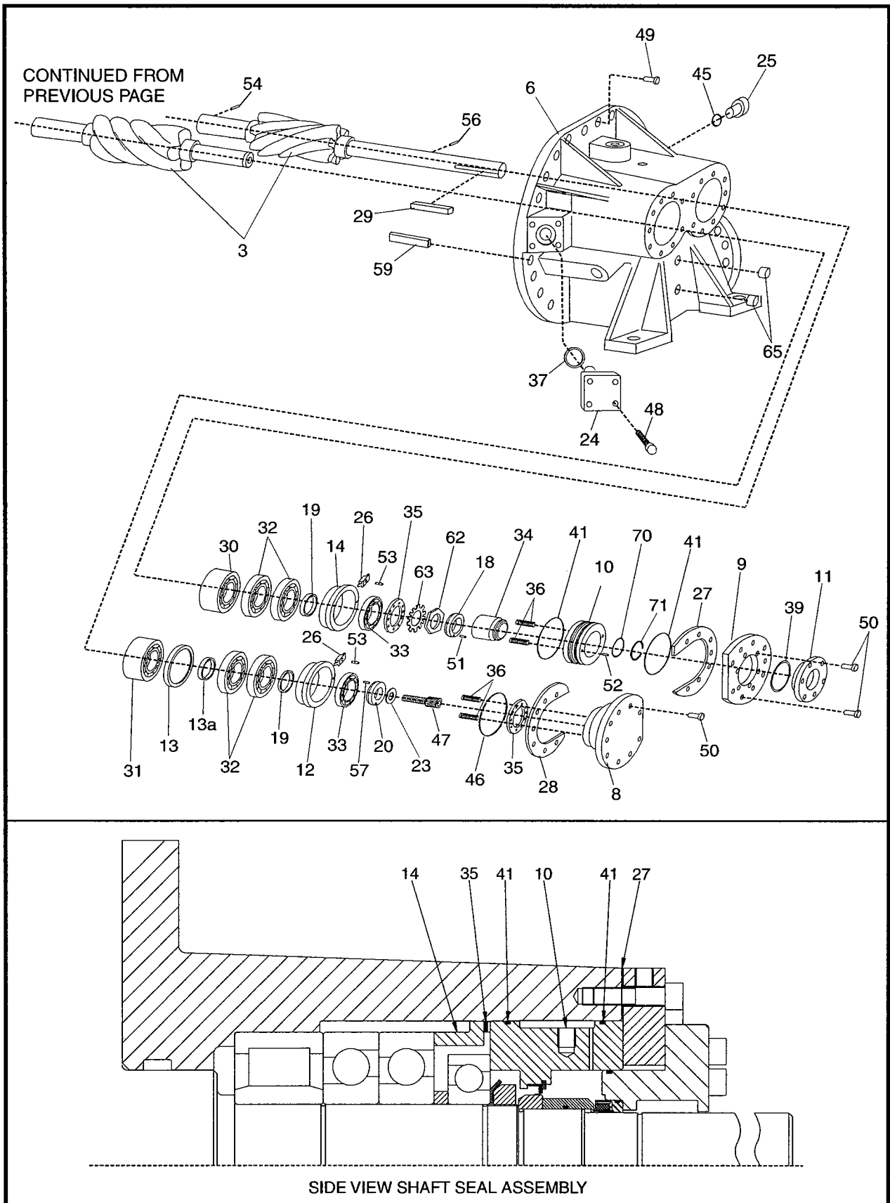
Figure 13b. Screw Compressor, TDSH 355.
