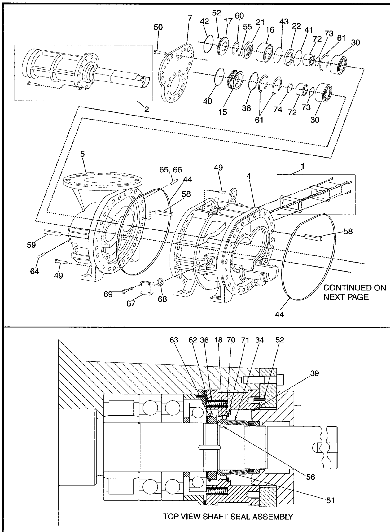
Figure 13a. Screw Compressor, TDSH 355.
