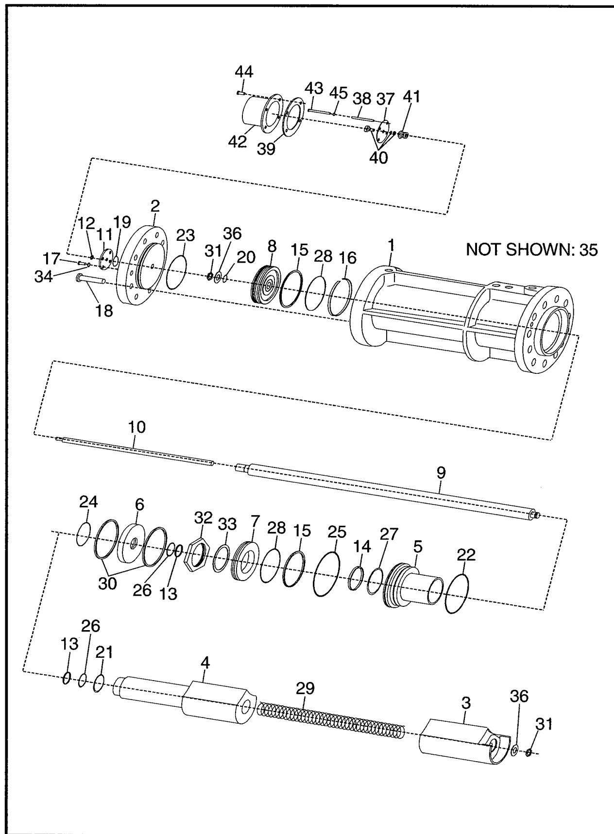
Figure 8. Slide Valve/Stop, 233.
