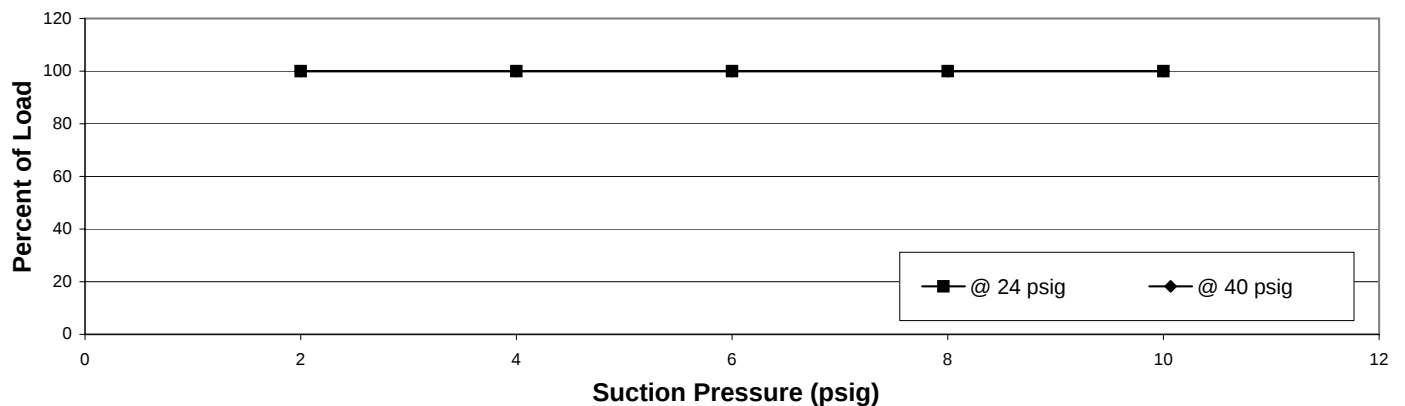
PERCENT COMPRESSOR LOAD
