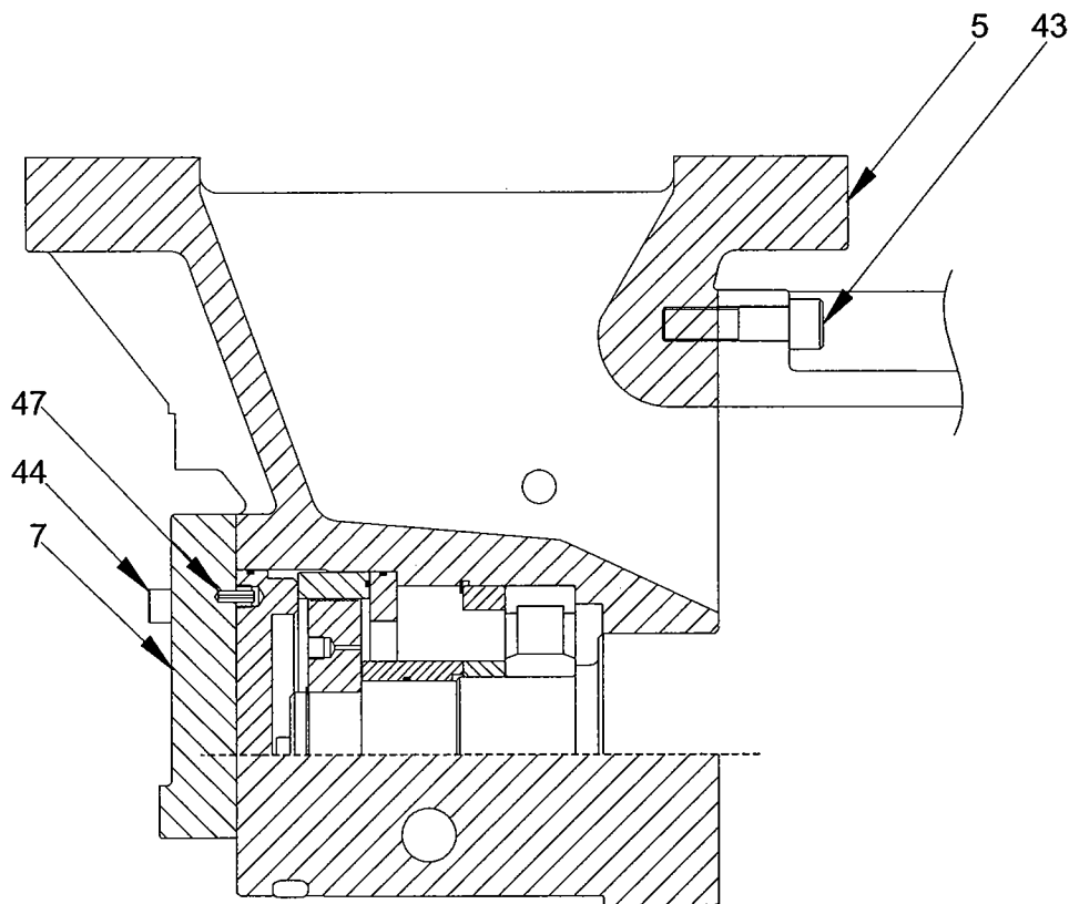
SIDE VIEW INLET CASING
