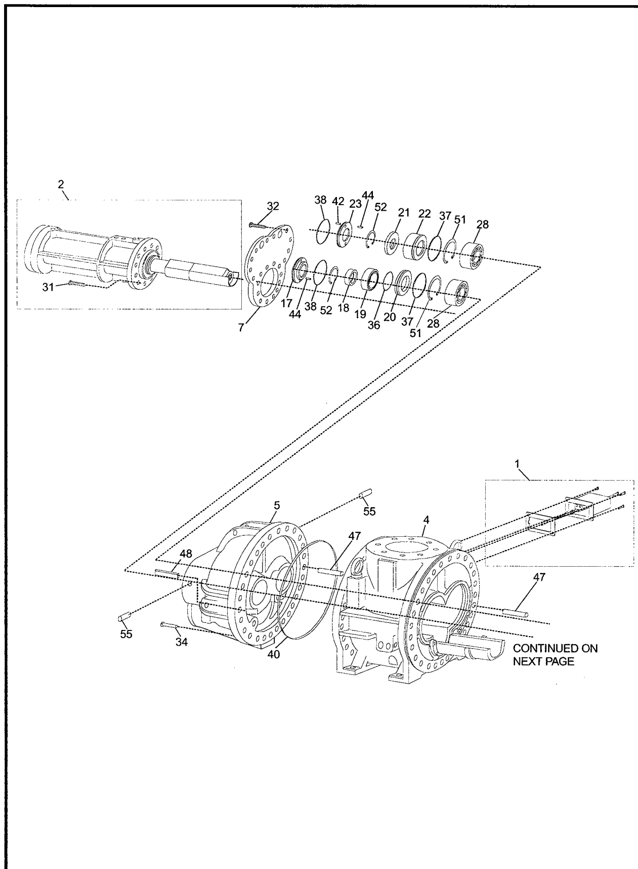
Figure 7a. Screw Compressor, 233.
