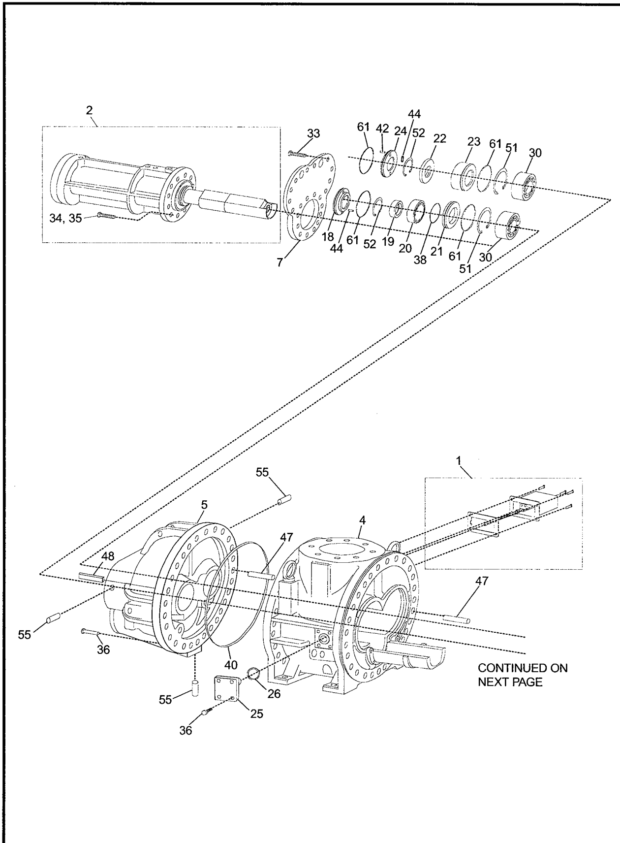
Figure 4a. Screw Compressor, 193.
