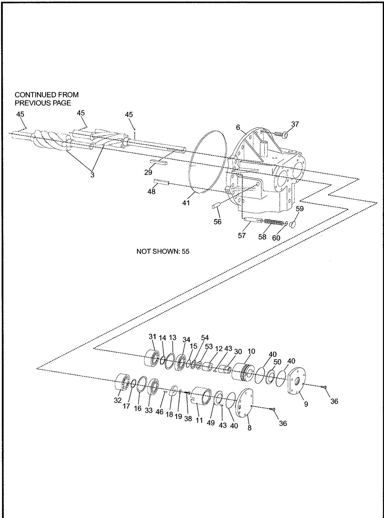
Figure 1b. Screw Compressor, 163.
