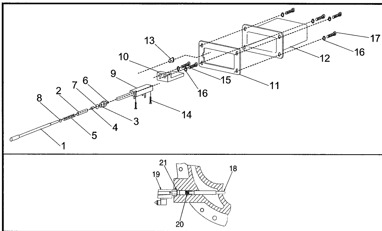
Figure 17. Slide Stop Indication Assembly, All Models.
