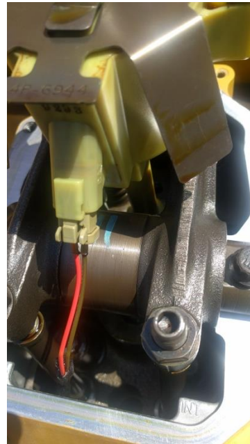
Tappet assembly under valve cover
