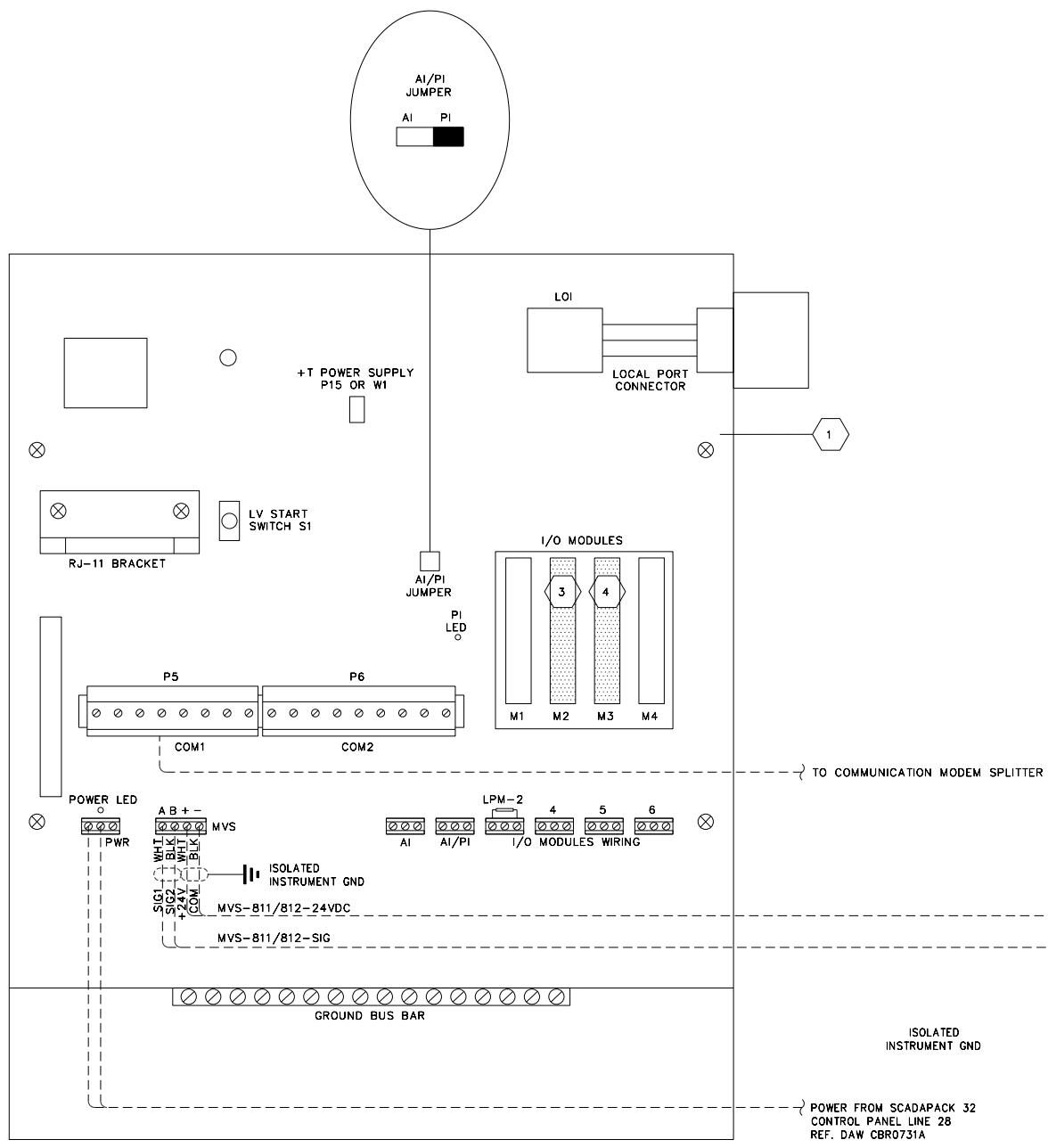
ROC407 FLOBOSS REMOTE OPERATIONS CONTROLLER LAYOUT
