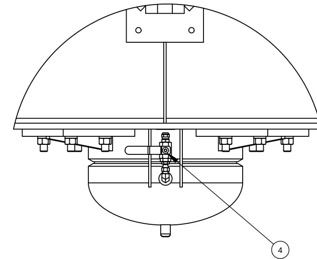
DETAIL C SCALE 1 : 10
