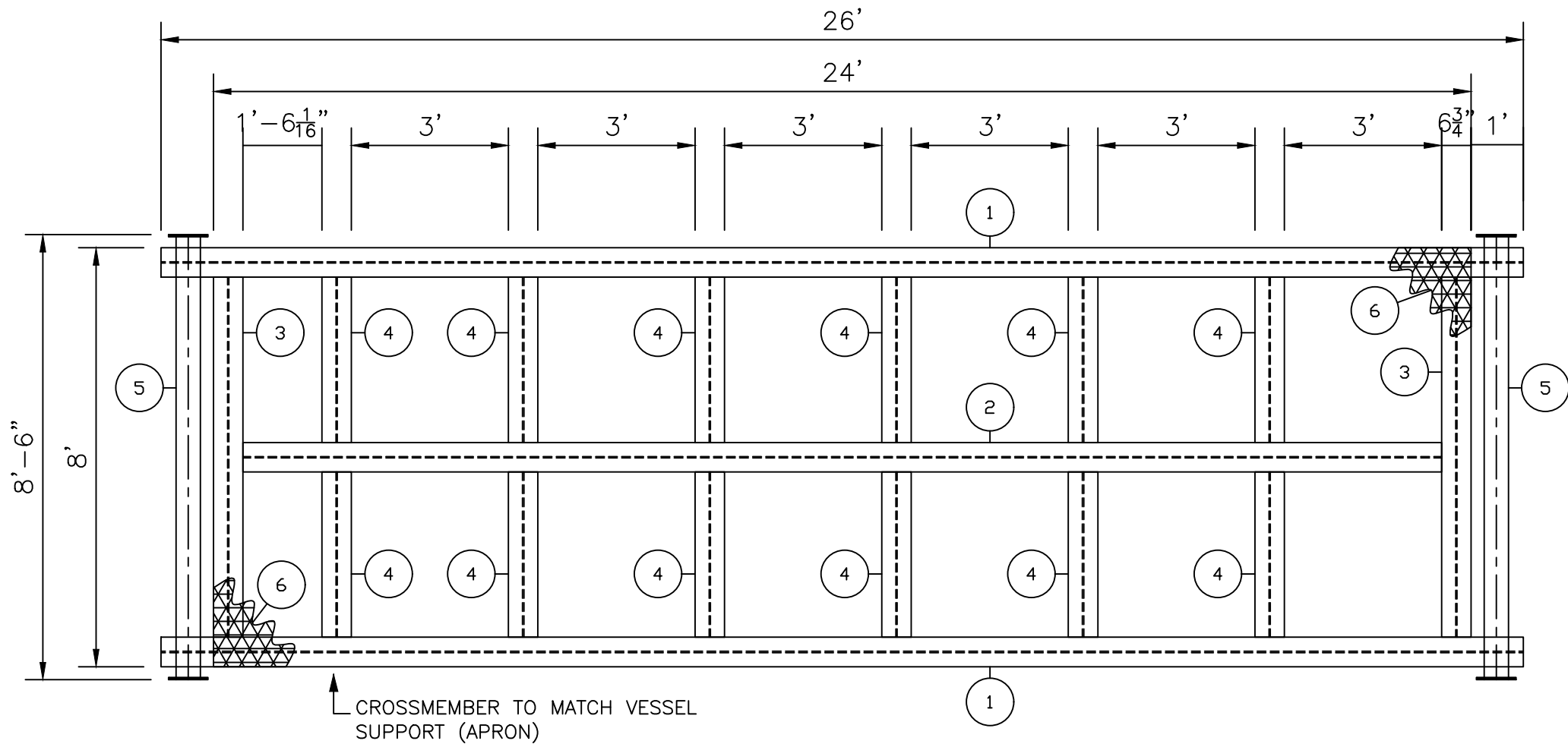
PLAN VIEW
