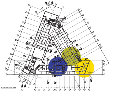
main floor
