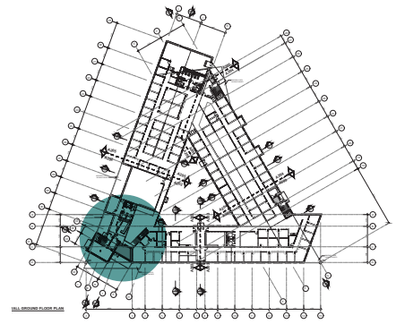
main floor
