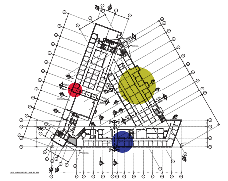
main floor
