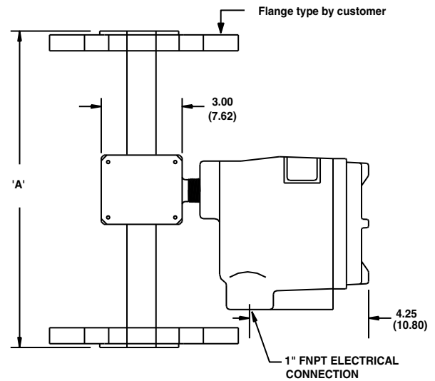
CLASSIC™ 832 In-Line Flanged (Vertical)
