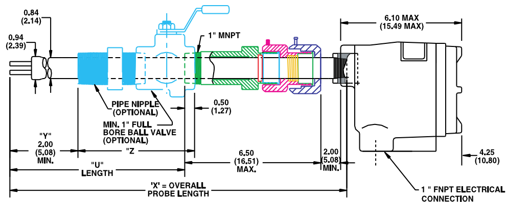
CLASSIC™ 816 Retractable Packing Gland Threaded – 1" MNPT – to 50 psi
