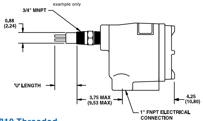
CLASSIC™ 810 Threaded
