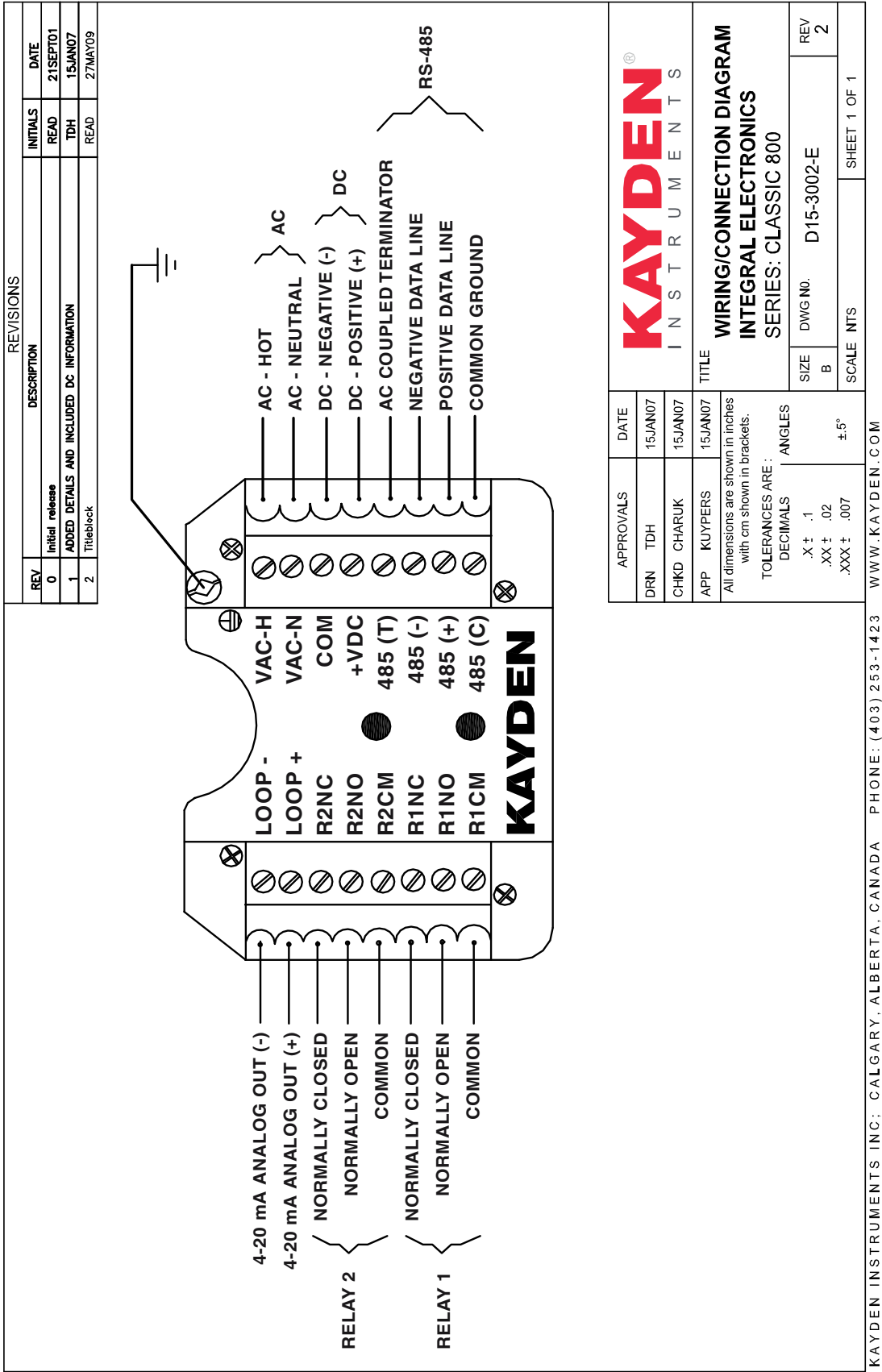
Figure 12 – CLASSIC 800 Wiring Connection Diagram
