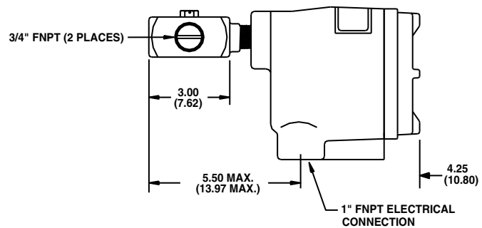
CLASSIC™ 830 In-Line Threaded (Horizontal)
