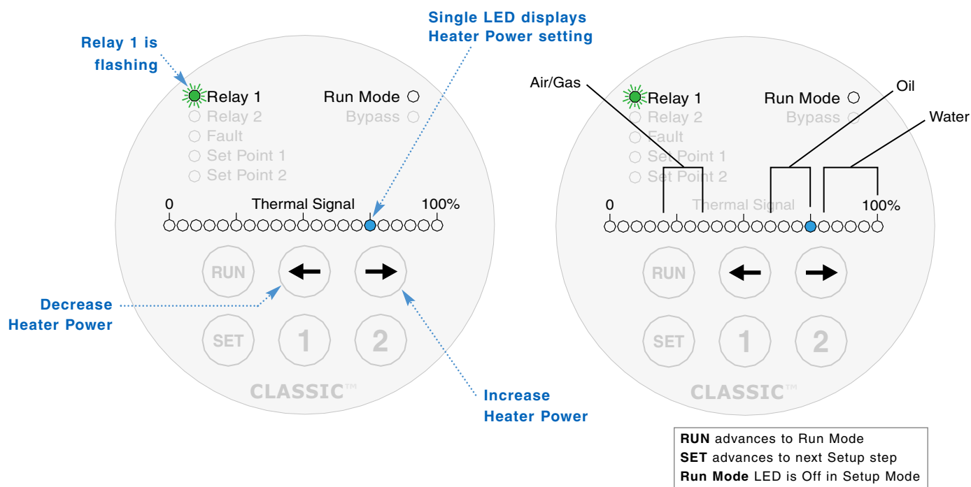
Figure 19 – Setting the Heater Power
