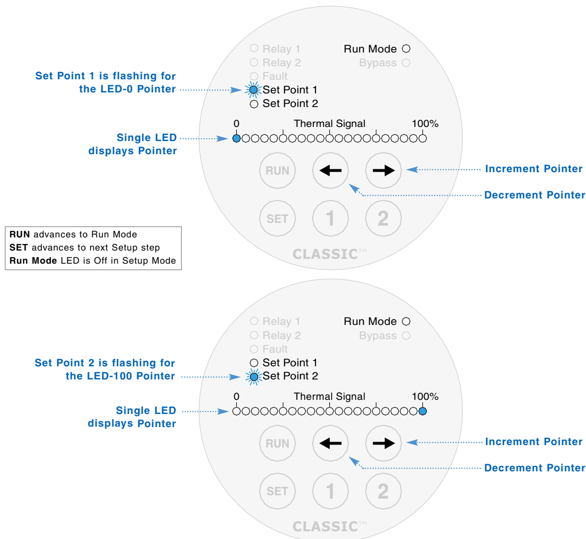
Figure 23 – Setting the 0% & 100% Thermal Signal
