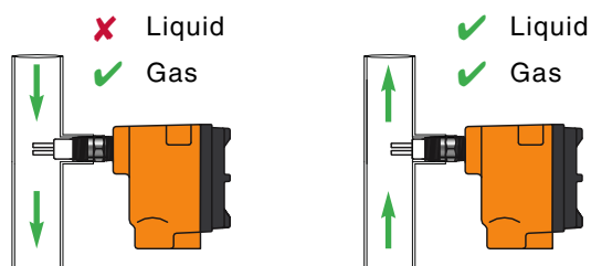
Figure 8 - Vertical Pipe, Flow Up & Down
