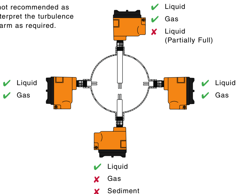
Figure 7 - Horizontal Pipe, Sensor Positioning
