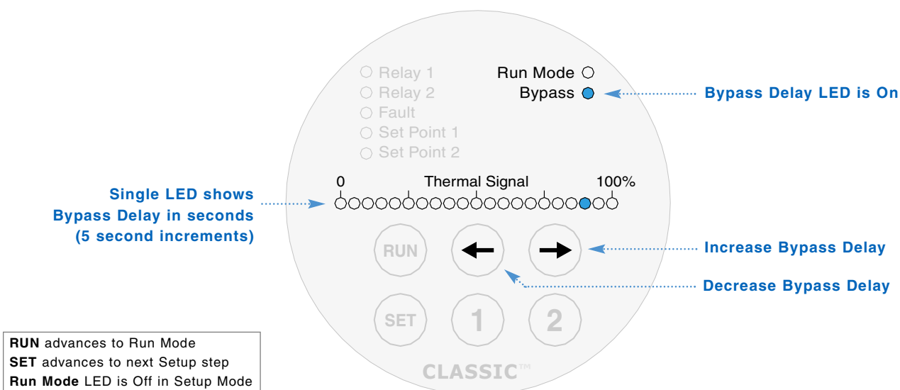
Figure 18 – Start-up Bypass Timer
