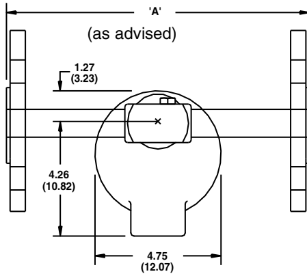
CLASSIC™ 832 In-Line Flanged (Horizontal)
