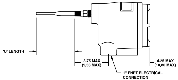
CLASSIC™ 821 Threaded (Single Probe)
