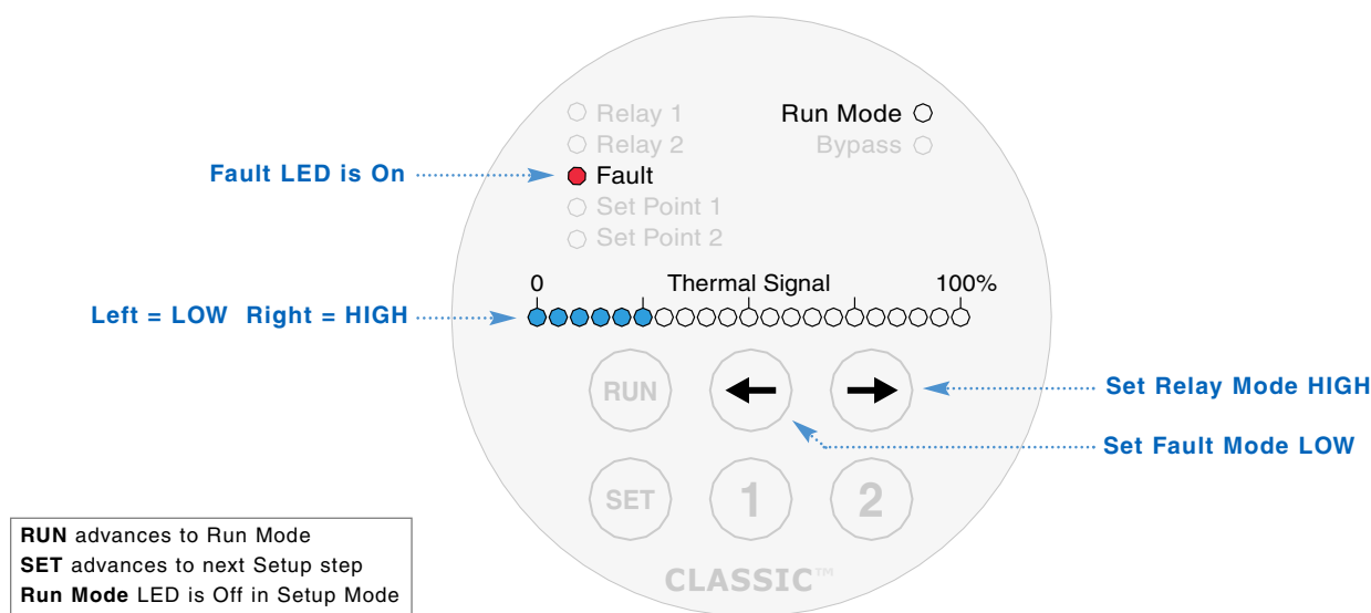
Figure 16 – 4-20 mA Fault Mode Configuration
