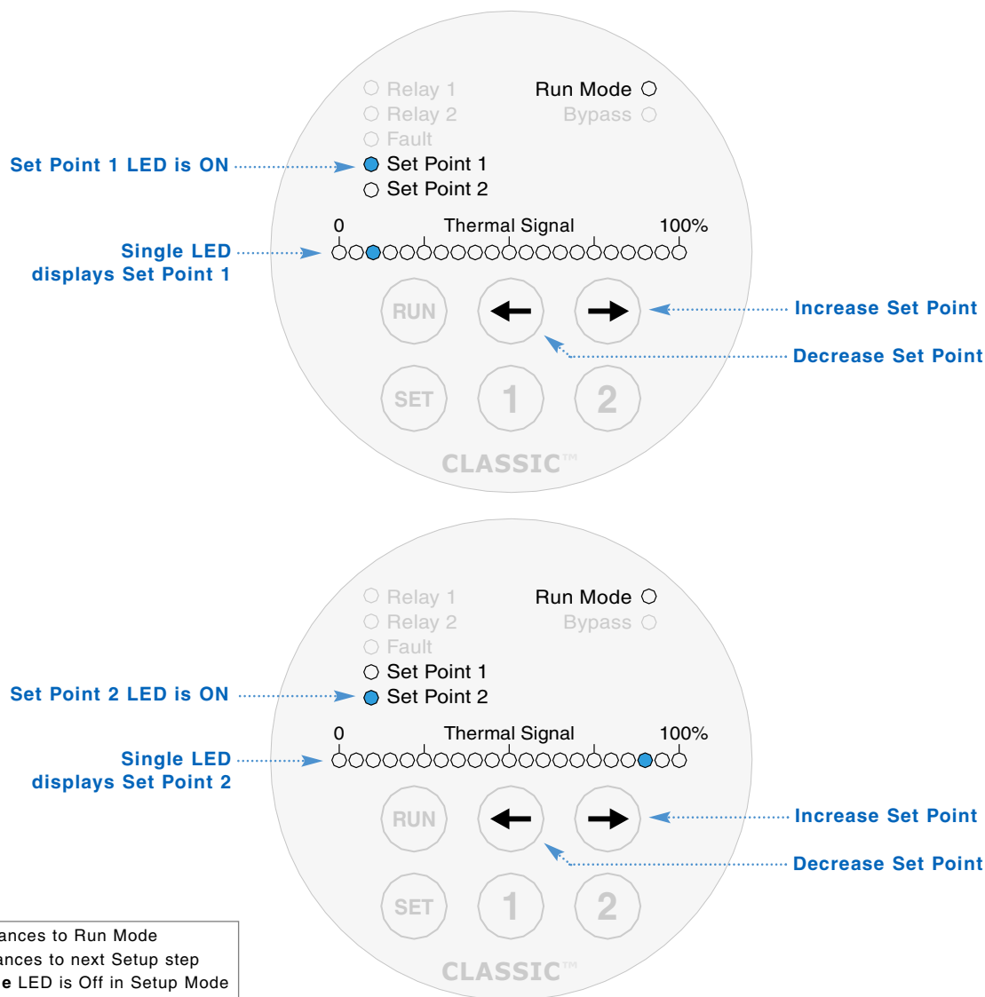
Figure 17 – Set Point 1 & 2 Configuration
