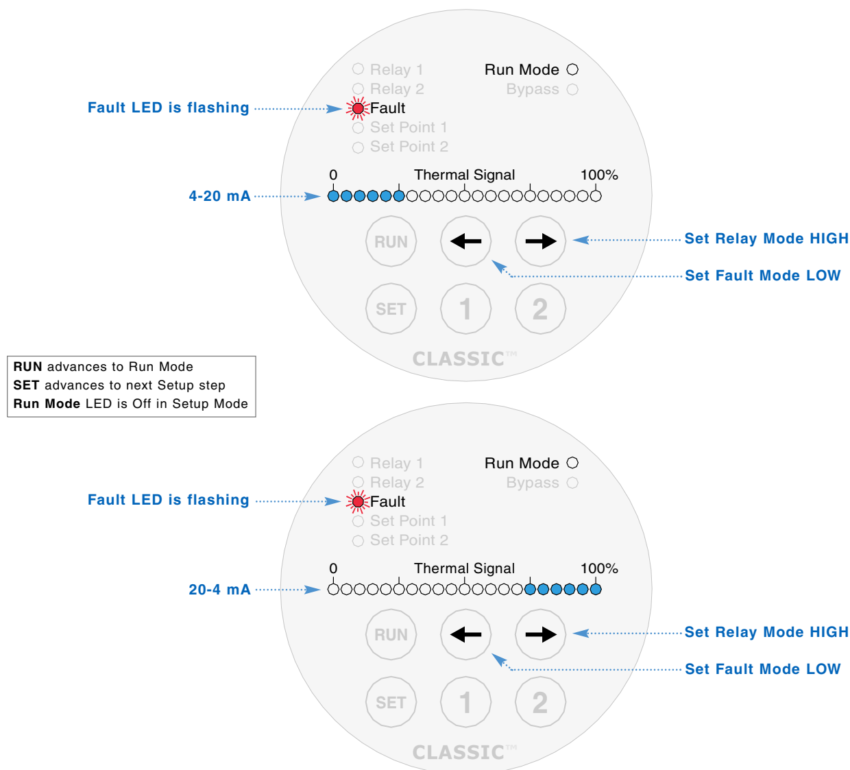
Figure 21 – 4-20 mA & 20-4 mA Output Mode
