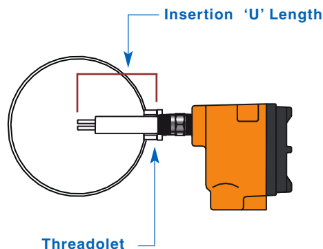
Figure 5 - Insertion 'U' Length
