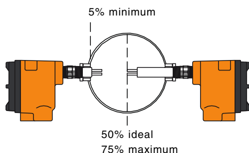
Figure 6a - Horizontal Pipe, Side Mounting
