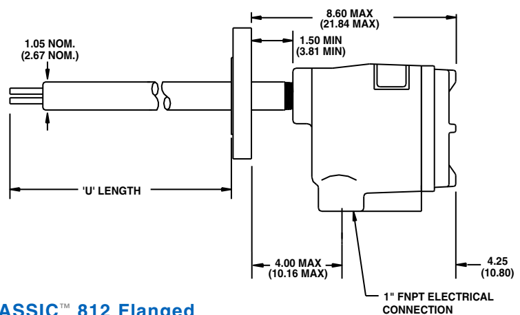
CLASSIC™ 812 Flanged
