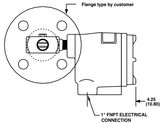
CLASSIC™ 832 In-Line Flanged (Horizontal)
