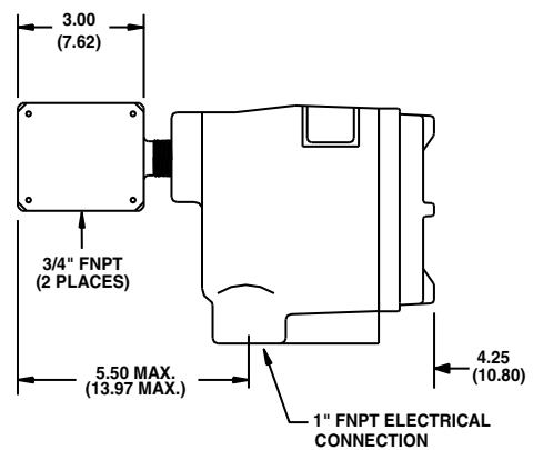
CLASSIC™ 830 In-Line Threaded (Vertical)
