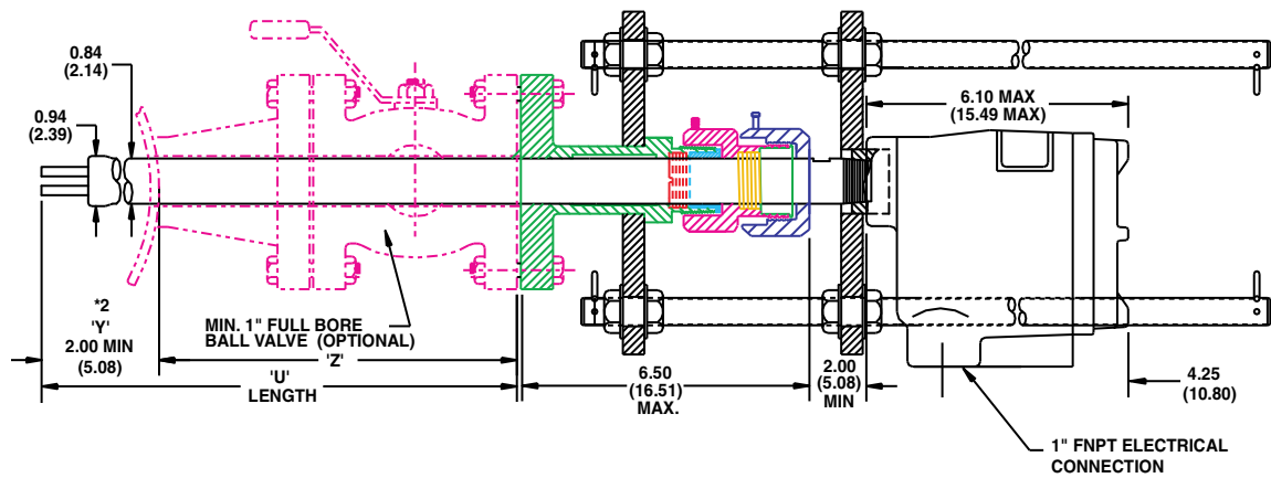
CLASSIC™ 814 Retractable Packing Gland Flanged – to 500 psi
