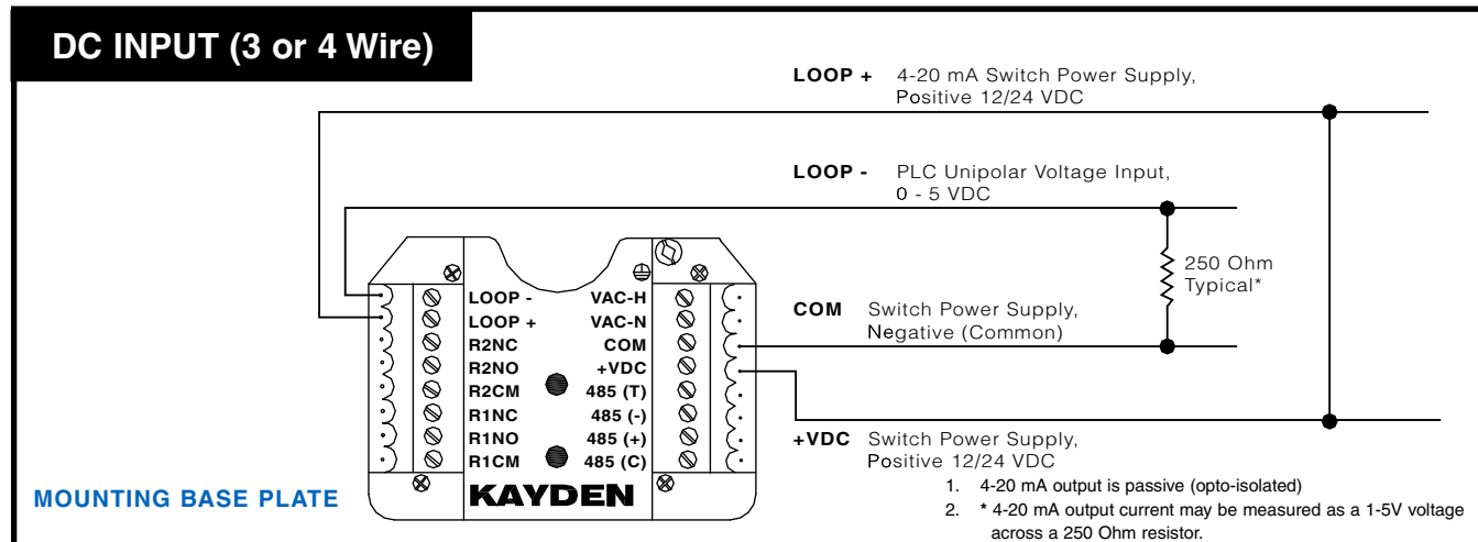
Figure 3 – 4-20 mA Wiring
