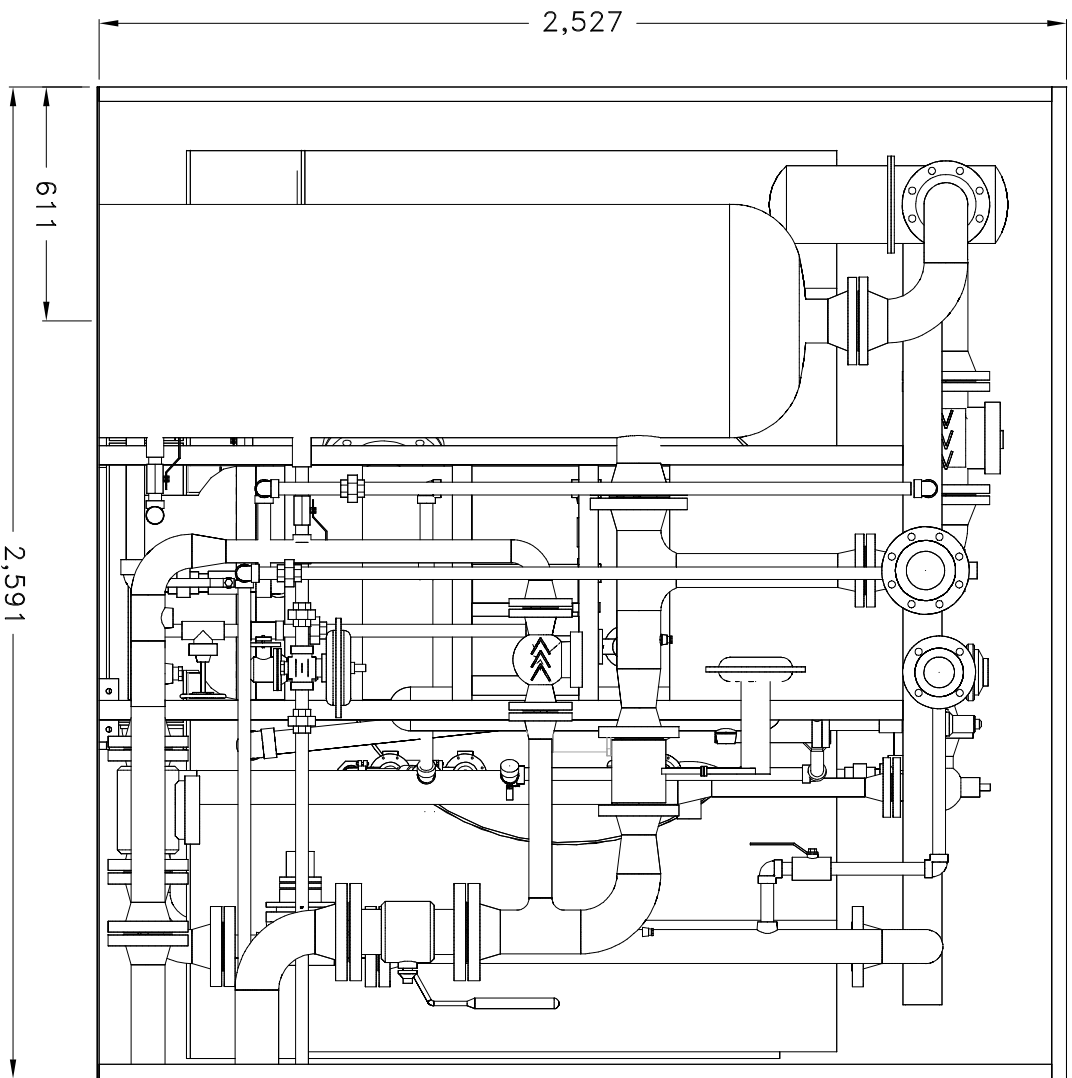
ELEV. VIEW 'D' SCALE 1:20
