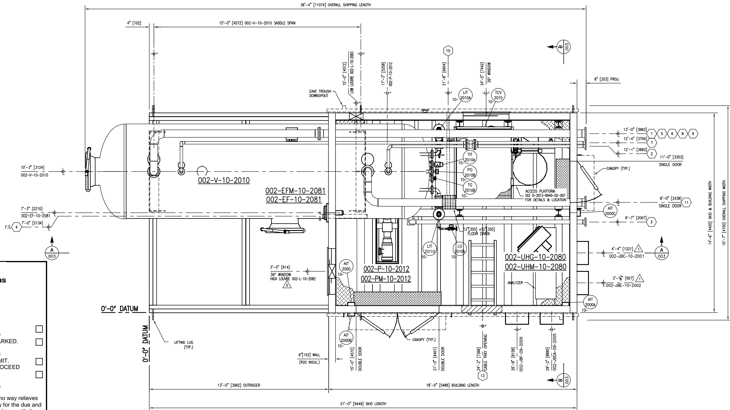
PLAN VIEW SCALE: 1/2"=1'-0"
