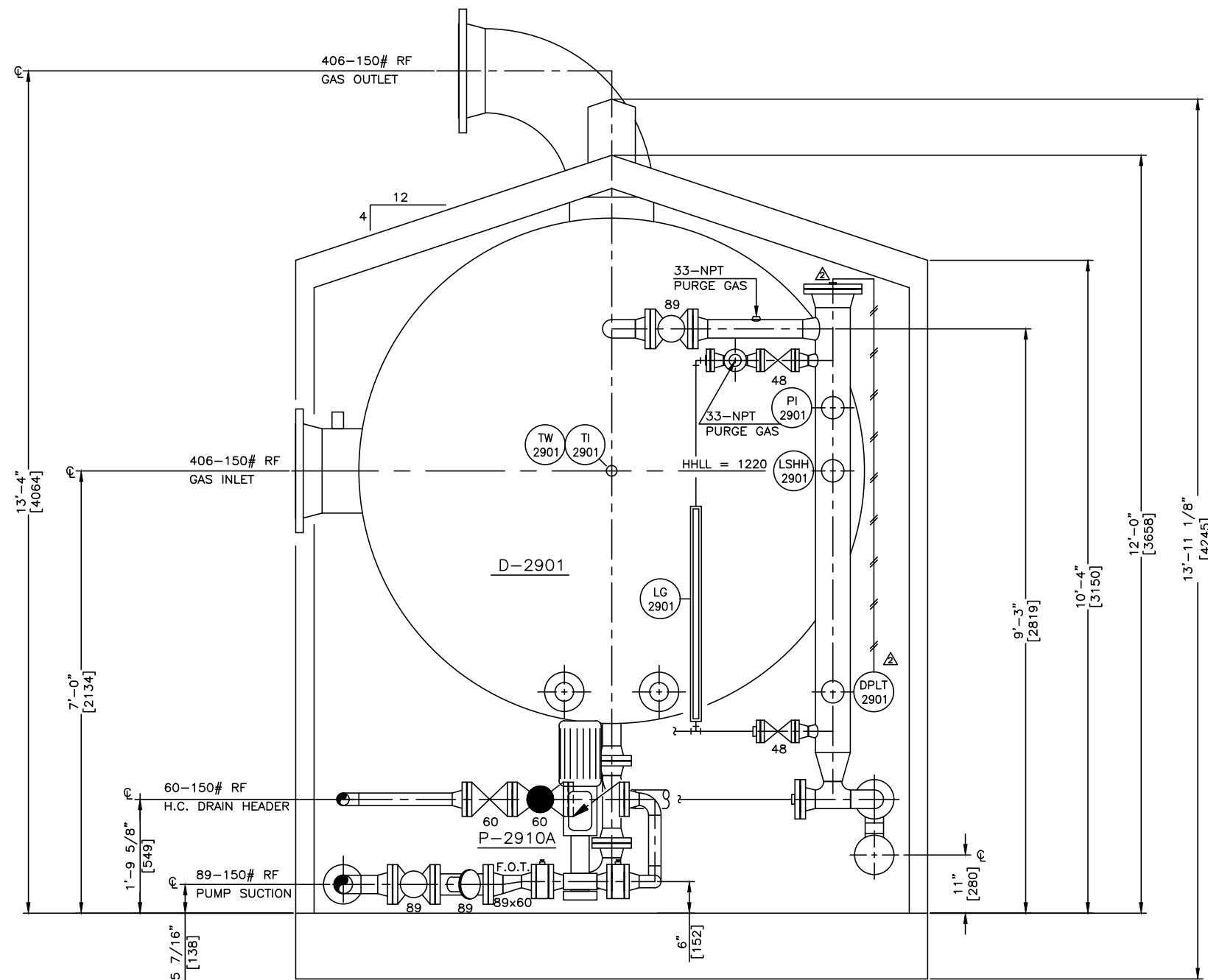
SECTION "A-A"
