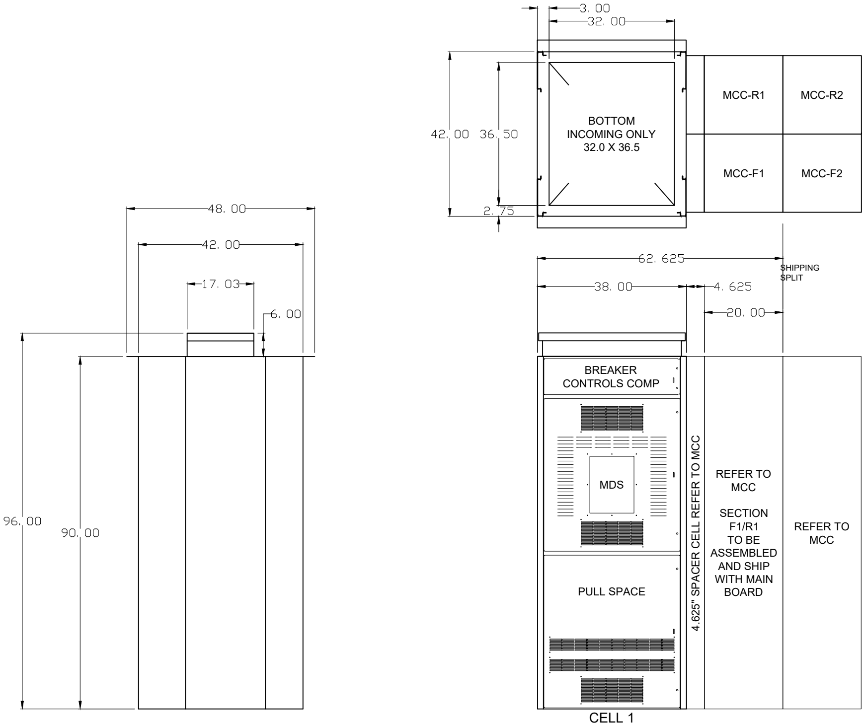
LEFT SIDE VIEW
