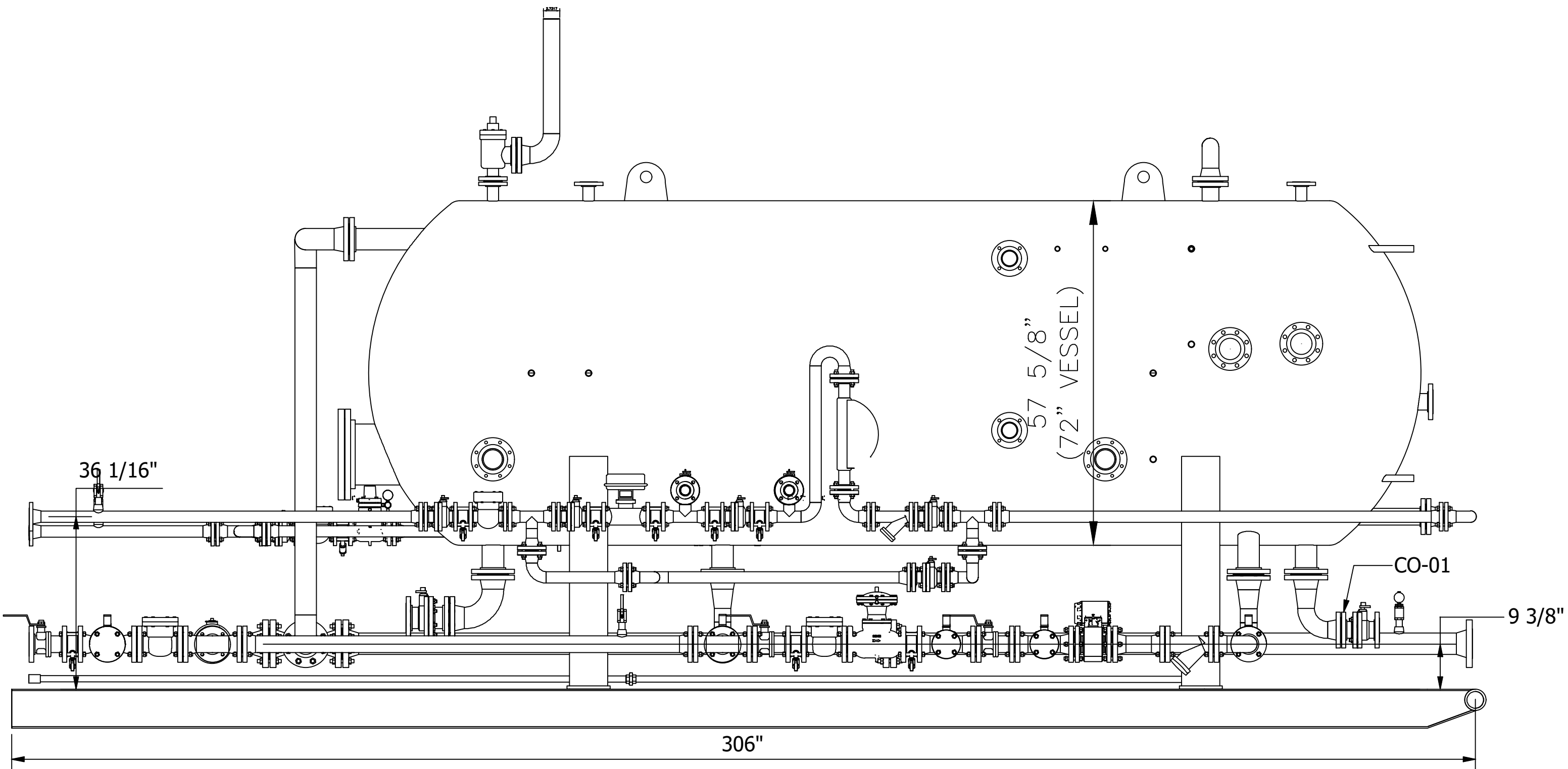
OIL & WATER PIPING - SIDE VIEW
