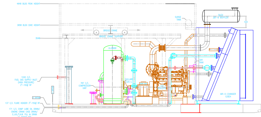
RIGHT SIDE ELEVATION NTS
