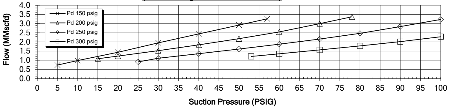
FLOW CURVE (flow rates guaranteed to +/- 5%)
