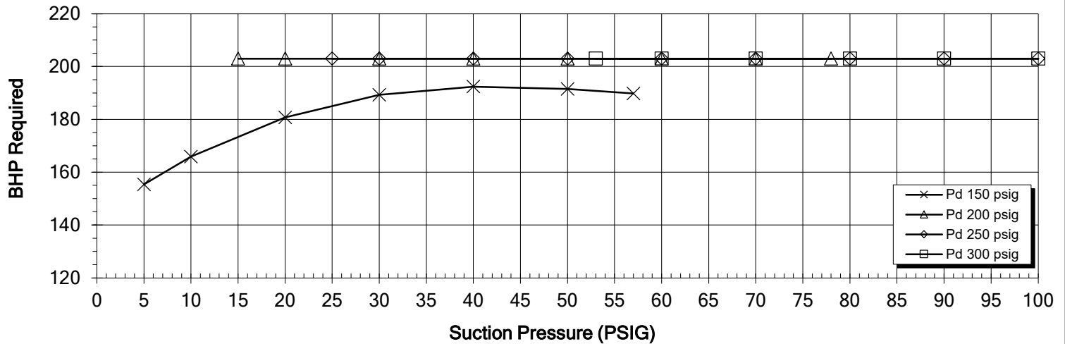
POWER CURVE
