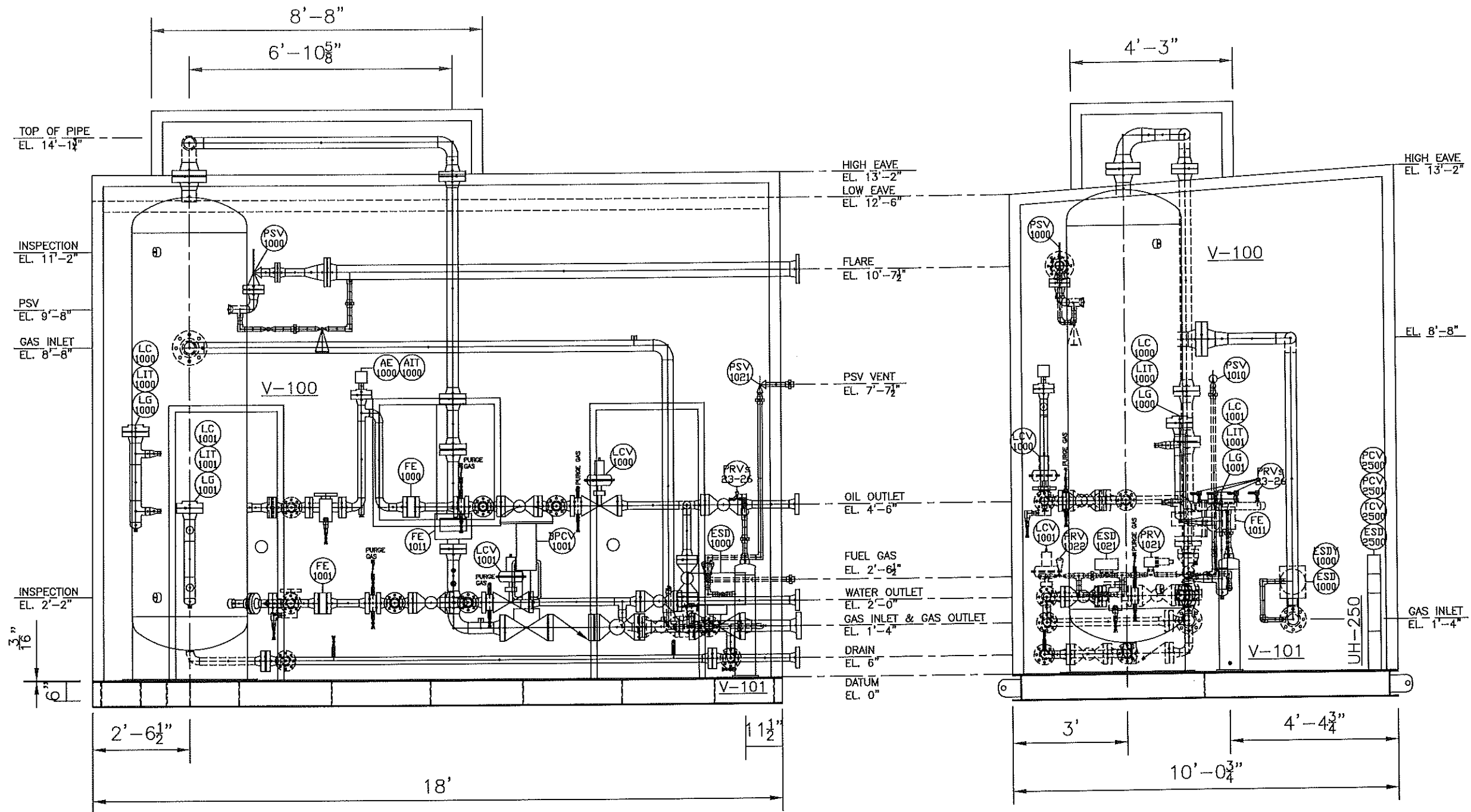
SIDE ELEVATION VIEW
