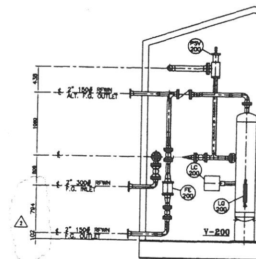
VIEW 'B-B'
