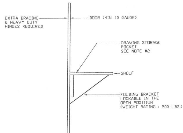
DETAIL '1'
