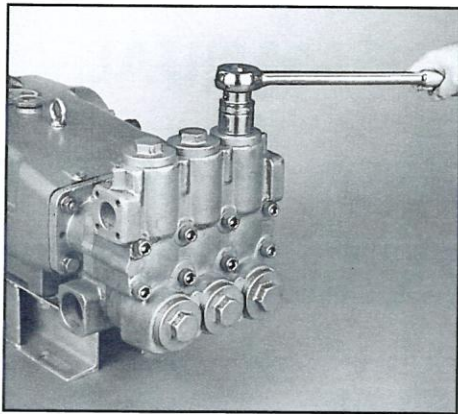
Removing Valve Plug (6760)
