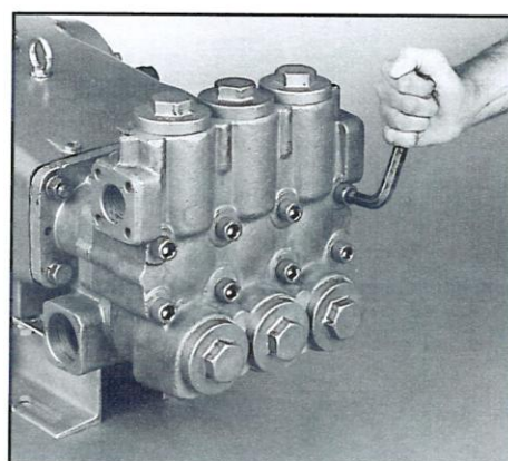
Removing screws from Discharge Manifold
