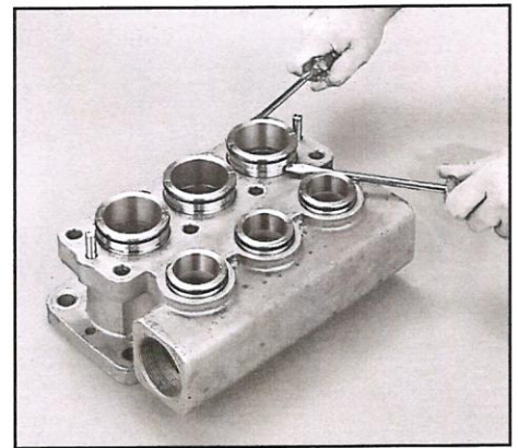
Removing V-Packing Spacer from Inlet Manifold
