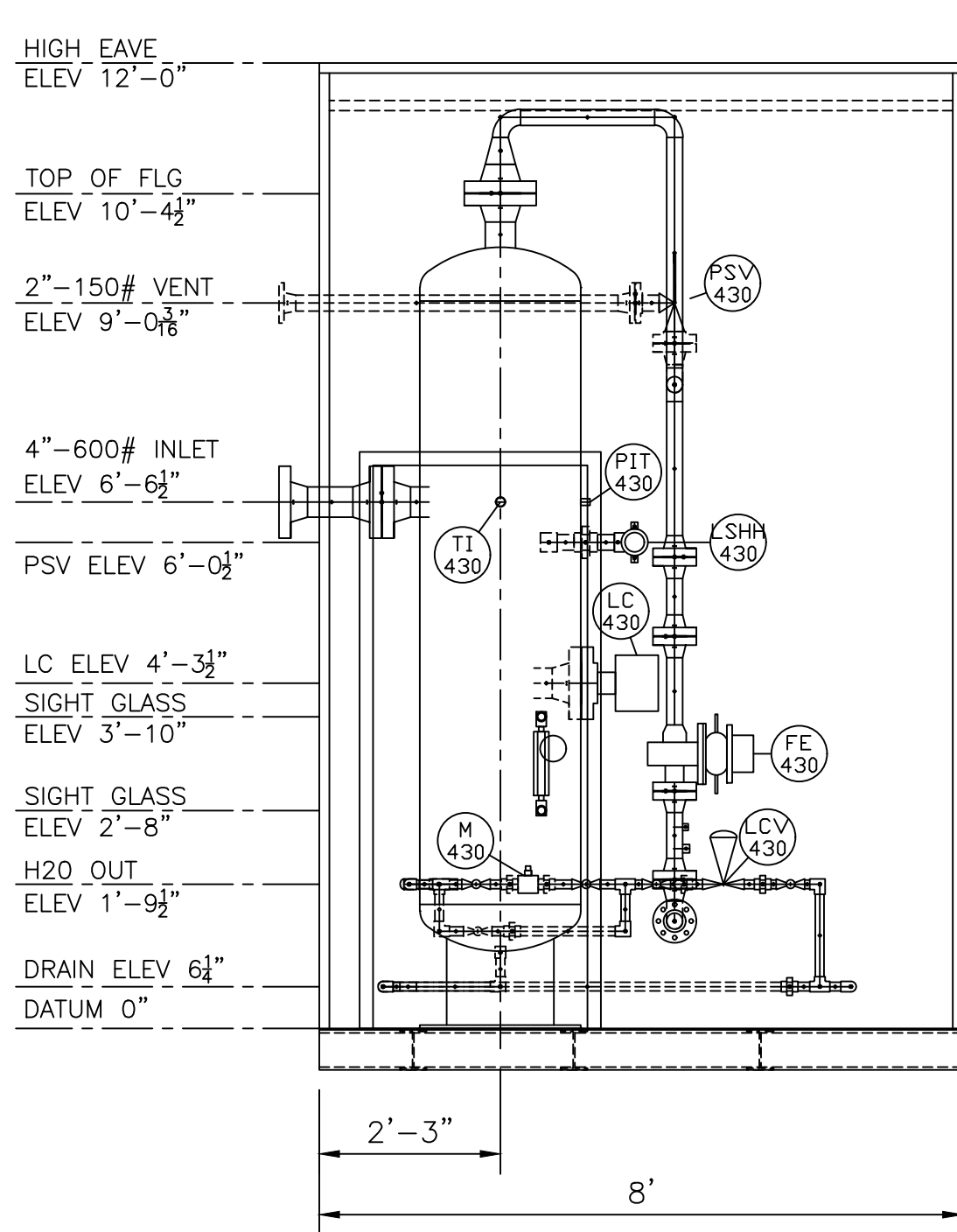
FRONT VIEW
