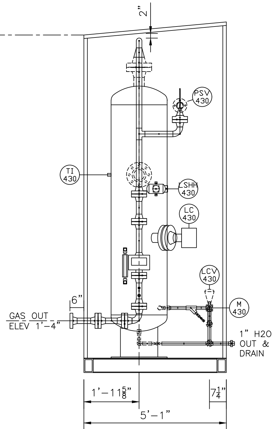
SIDE VIEW
