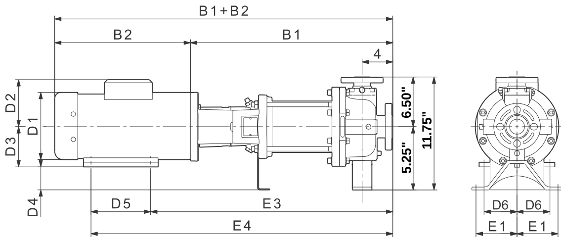
Dimensional sketches GA (1.5" x 1" x 6", 1.5" x 1" x 8")
