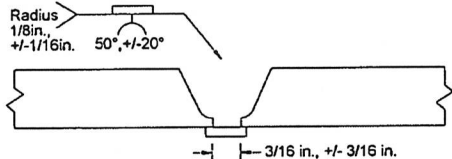
Figure 8 Single U Butt with Backing Strip
