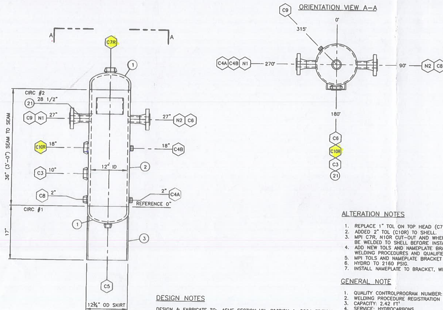
ELEVATION VIEW
