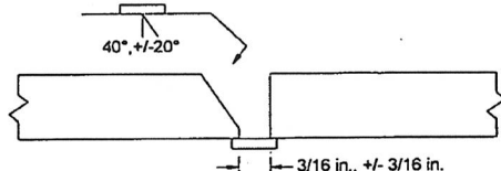
Figure 14 Single Bevel Butt with Backing Strip
