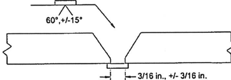
Figure 5 Single Vee Butt with Backing Strip
