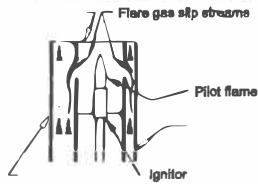
SLIP STREAM DETAIL scale 1:20
