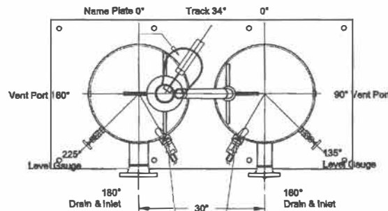
TOP VIEW: Orientation View scale 1:20
