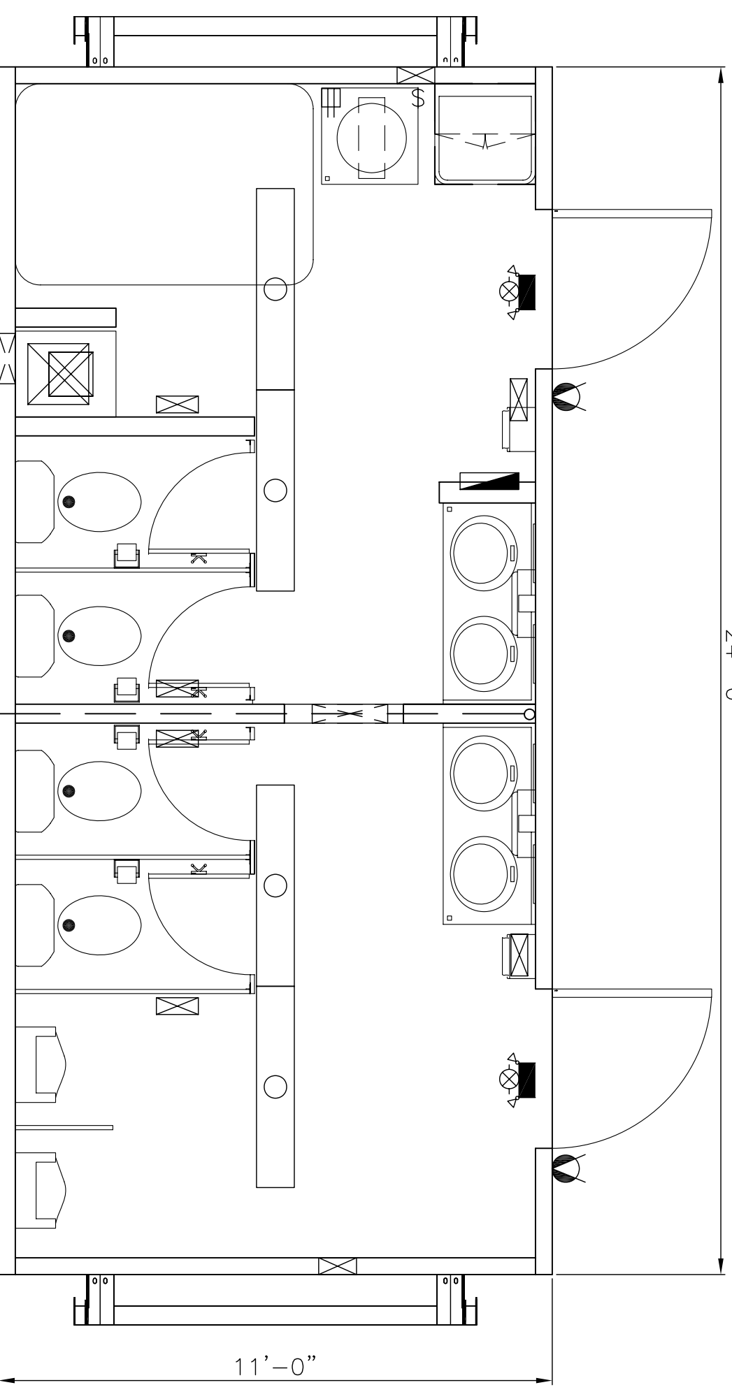
1 FLOOR PLAN A01 CEILING HEIGHT: 8'-0 1/4"
