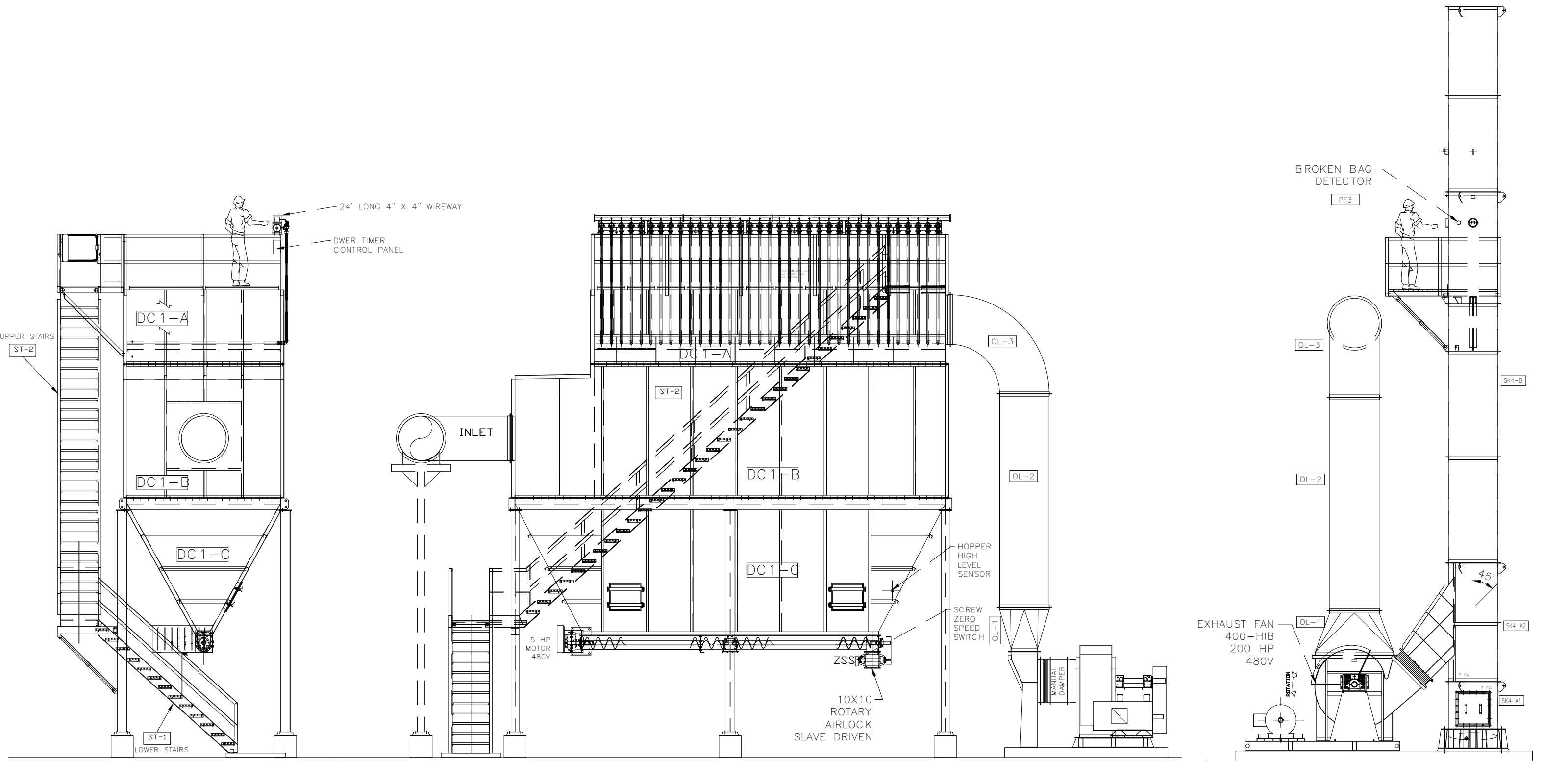
END VIEW
