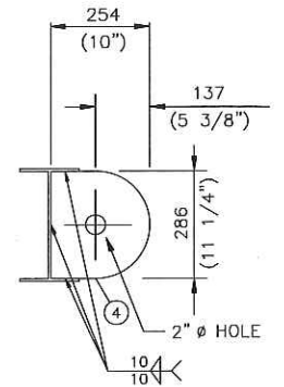
LIFT LUG DETAIL
