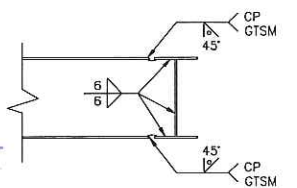
BEAM TO BEAM CONNECTION
