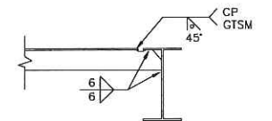
ANGLE TO BEAM CONNECTION
