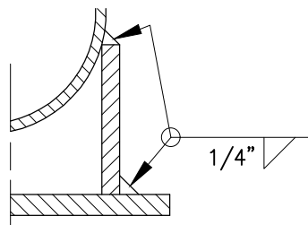
WELD DETAIL 1 WPS: AER-5/11
