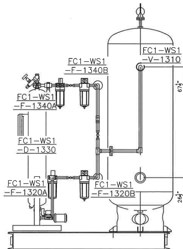
SECTION A-A SOME DETAILS OMITTED FOR CLARITY
