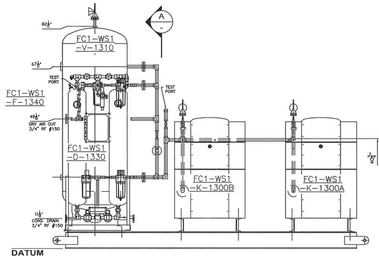
ELEVATION SOME DETAILS OMITTED FOR CLARITY
