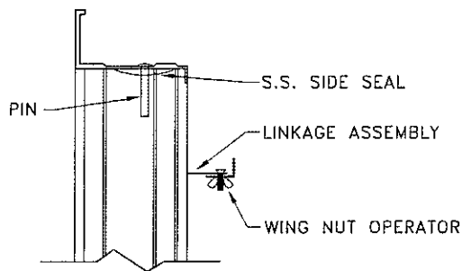
TOP VIEW (PARTIAL)
