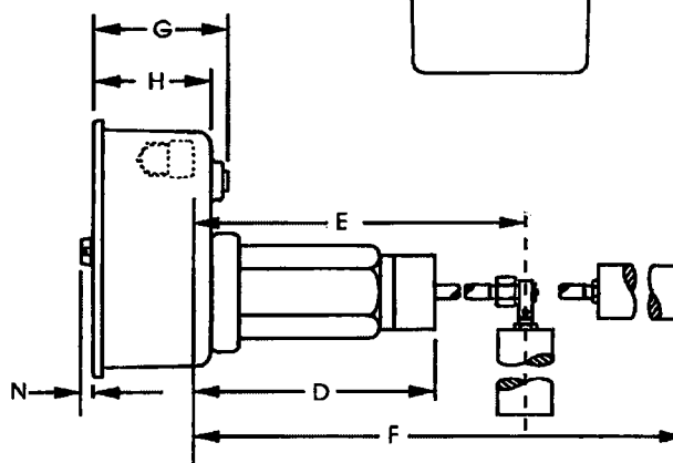
Side View of 1001XL
