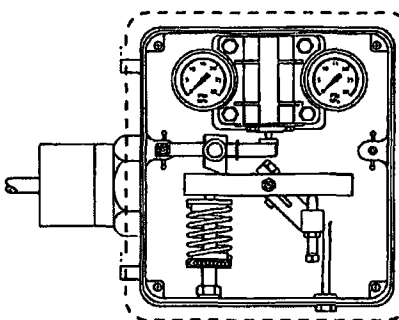
LEFT HAND MOUNT
