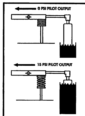
TOP LEVEL CONTROL
