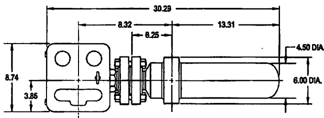
with Flanged Level Controller
