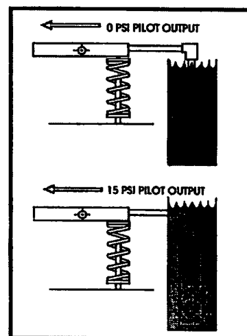
LIQUID INTERFACE CONTROL
