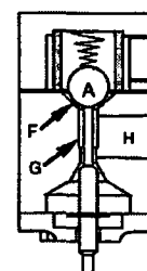
Relief Pilot
