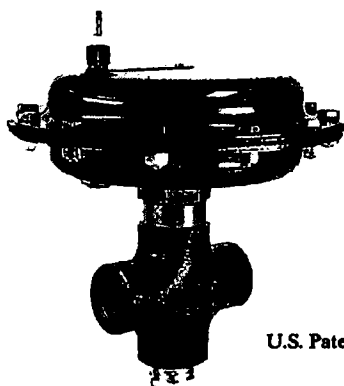
NON-ADJUSTABLE CONFIGURATION PLUGGED FOR GLOBE FLOW
