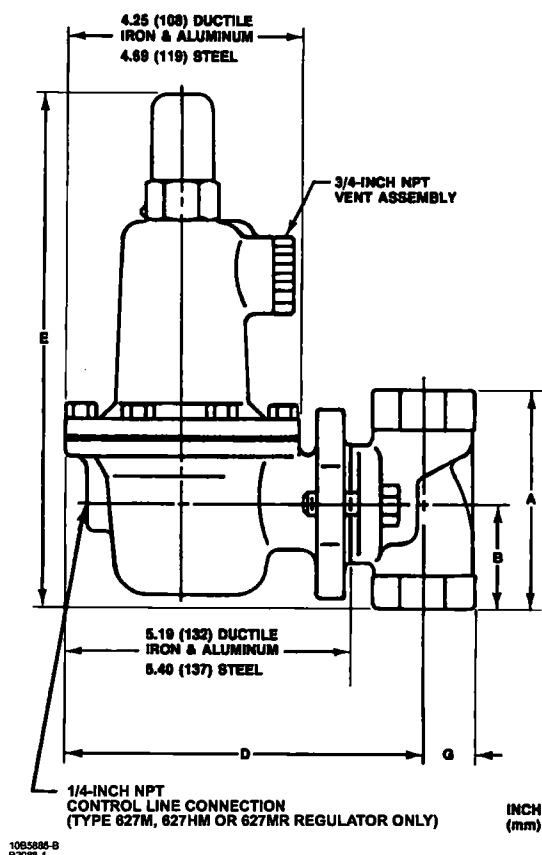
TYPES 627, 627R, 627M, AND 627MR SCREWED BODY
