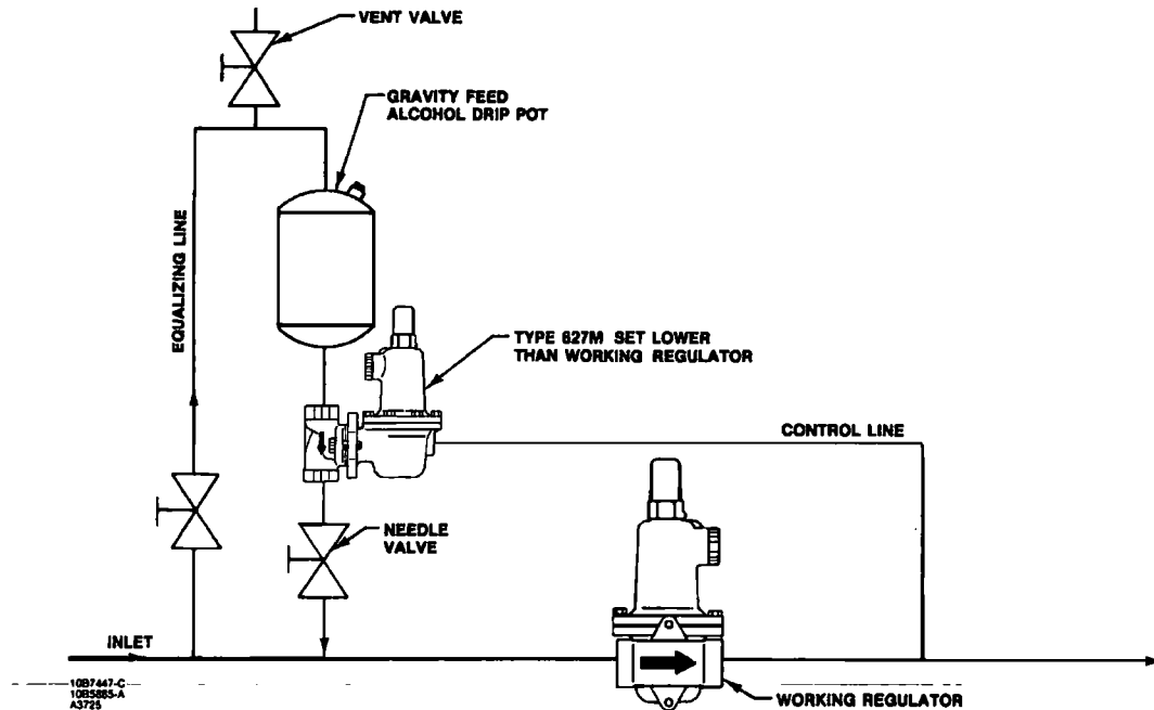
Figure 9. Schematic of De-Icer System
