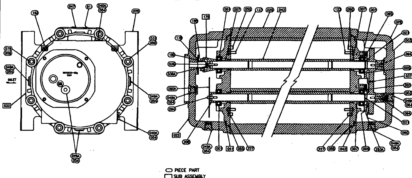
DETAIL TEMP. COMP. WELL
