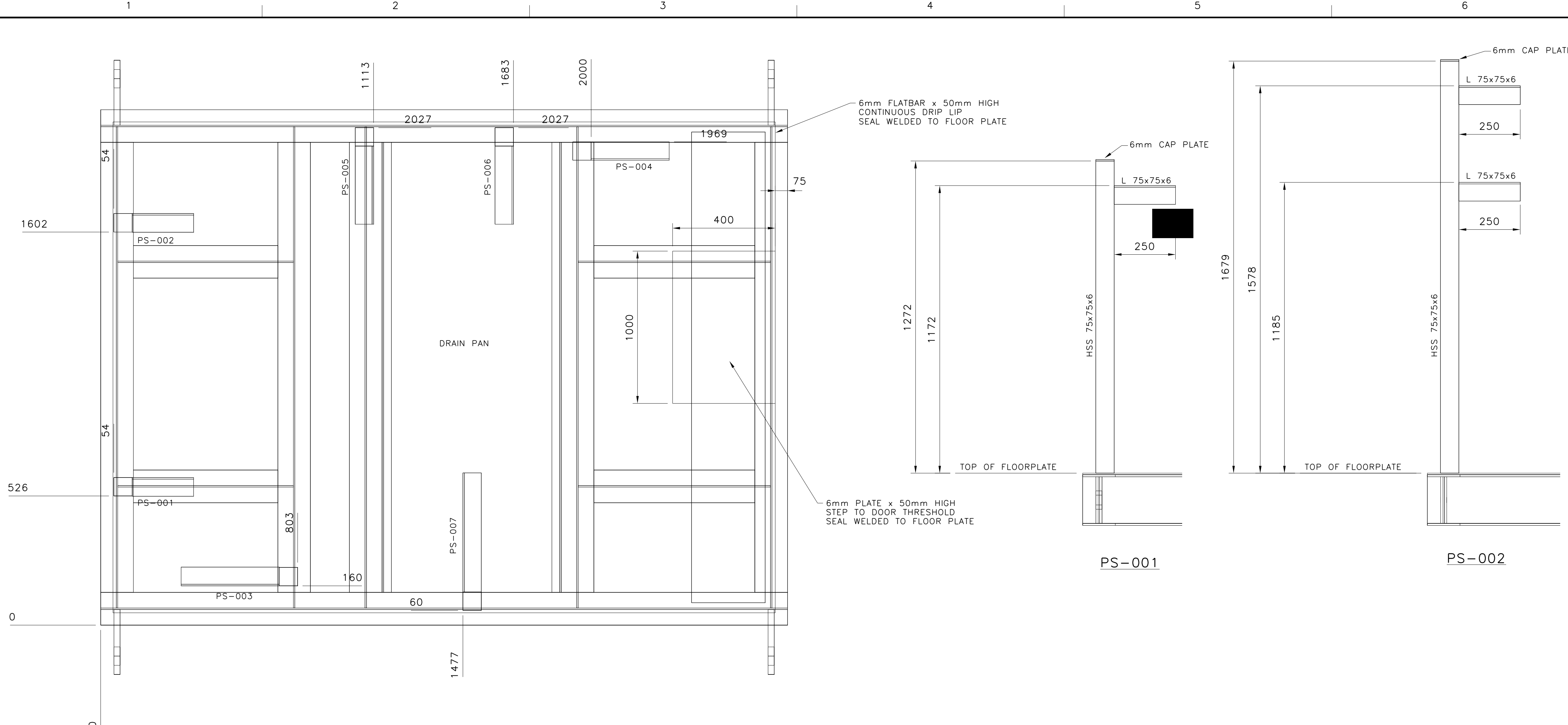
PIPE SUPPORT PLAN
