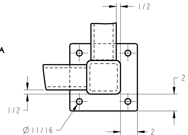
DETAIL A (TYP. 4 PLACES) SCALE 0.150
