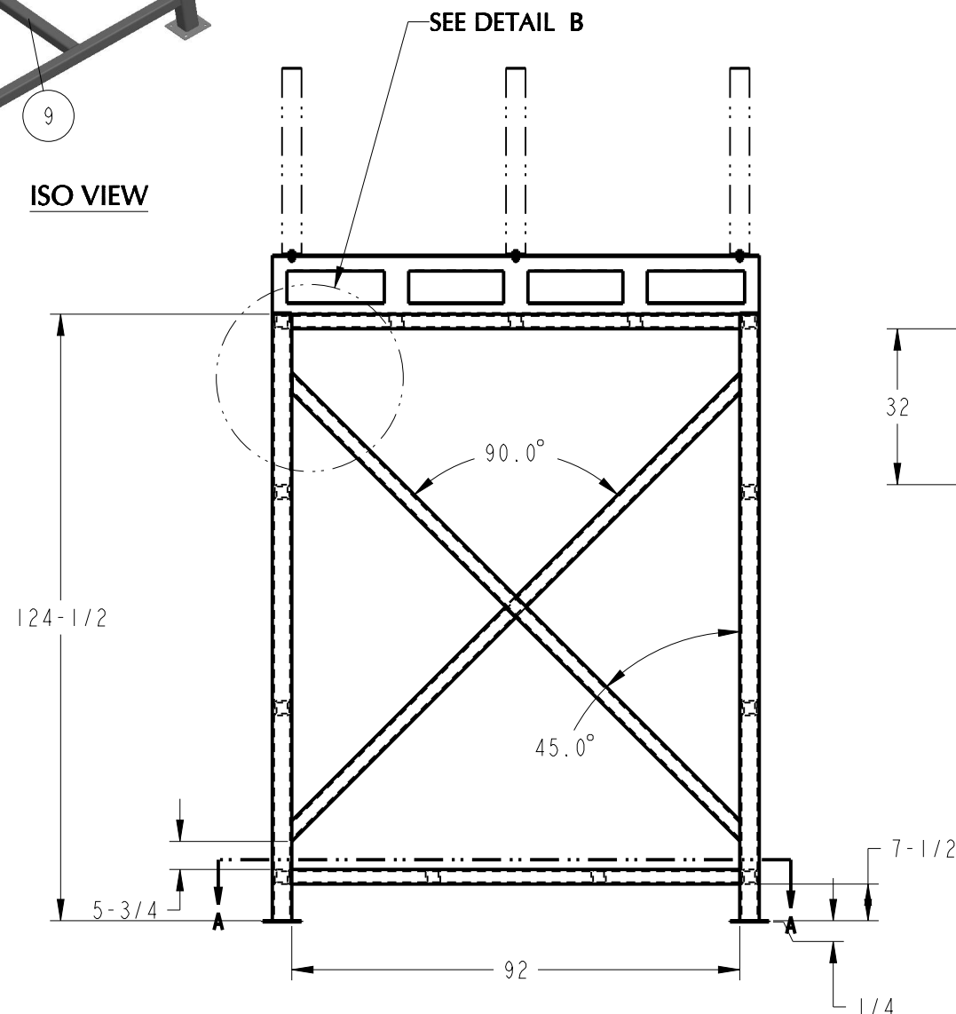
SIDE VIEW
