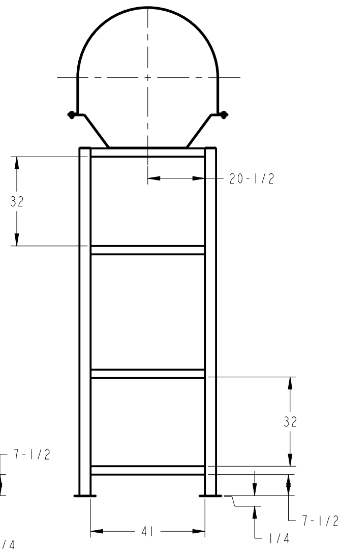
END VIEW
