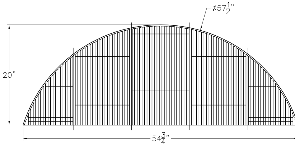
VANE ONLY INLET VIEW
