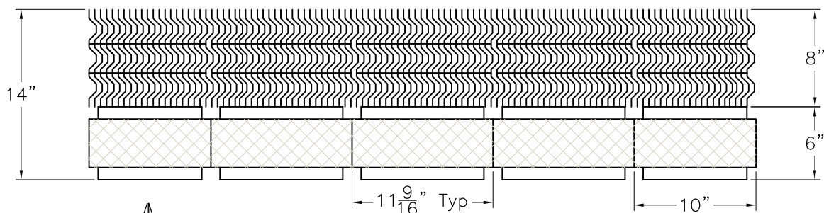
MESH-VANE ASSEMBLY TOP VIEW
