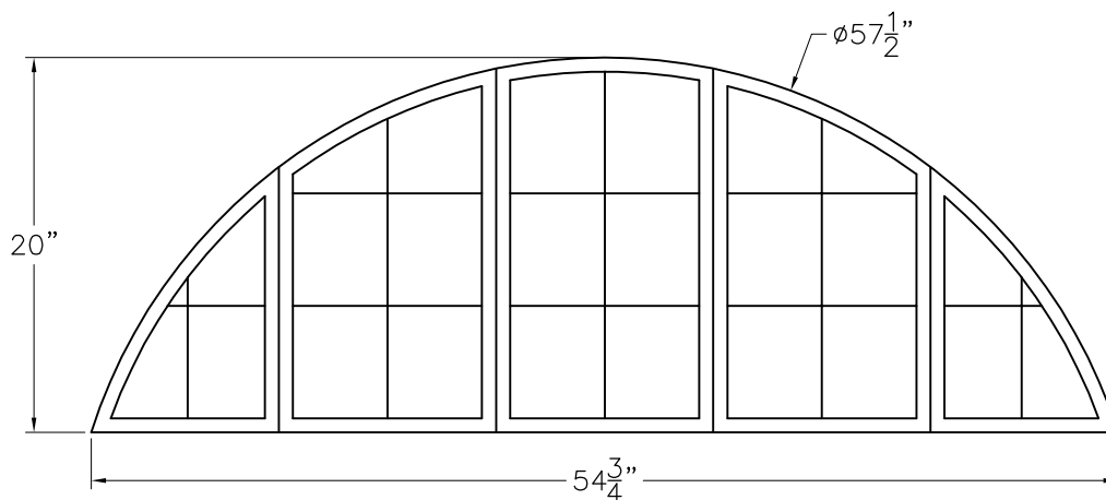
MESH ONLY INLET VIEW
