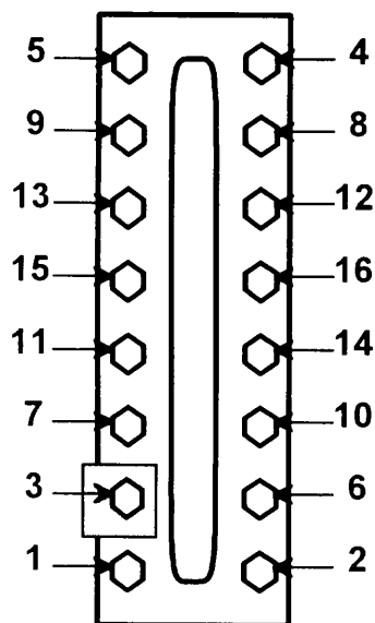
Nut Loosening Sequence Figure 3
