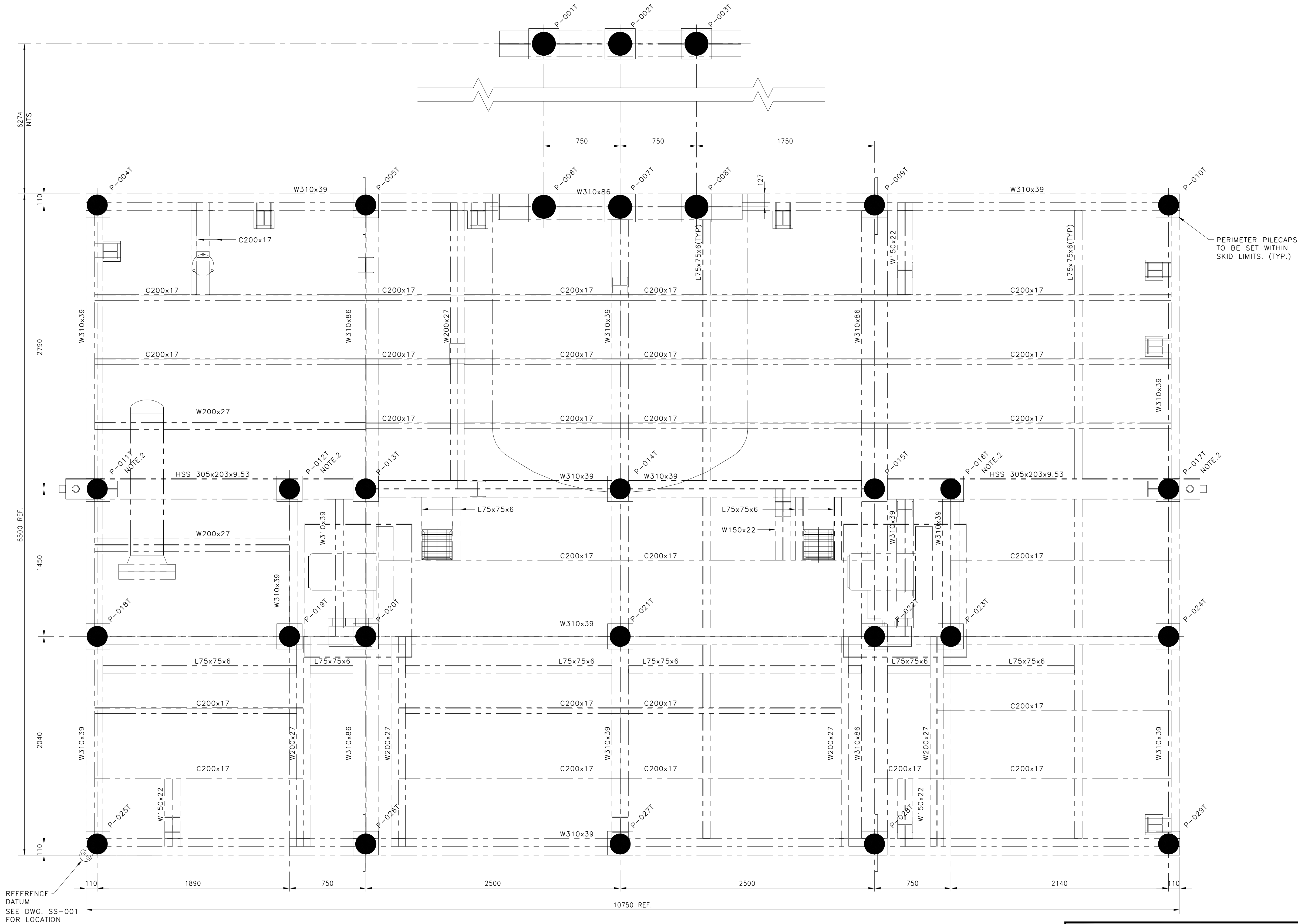
SEPARATOR/ SLUG CATCHER SKID - PLAN
