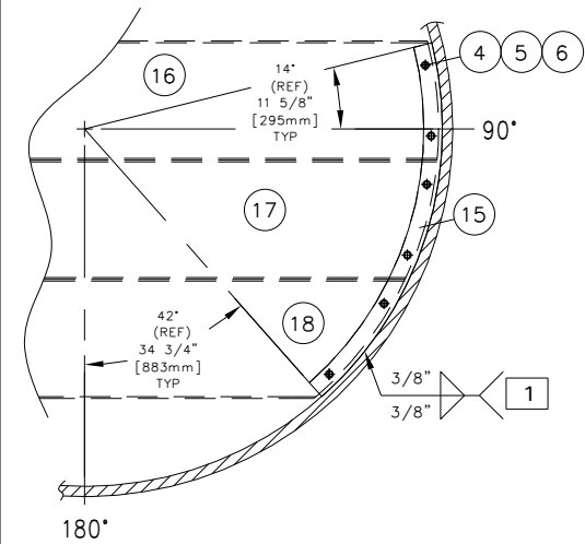
BAFFLE ITEM #2 DETAILS
