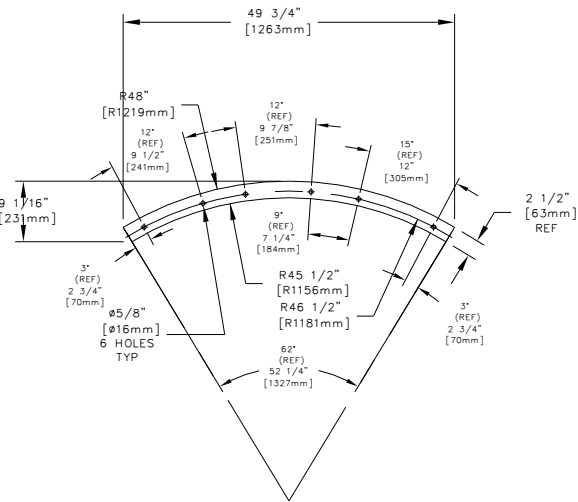
ITEM #15 CUTTING DETAILS 4 REQ'D
