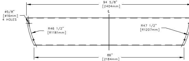
ITEM #17 CUTTING DETAILS 2 REQ'D
