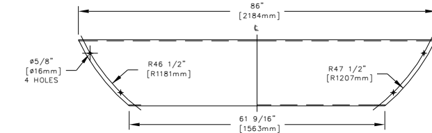
ITEM #18 CUTTING DETAILS 2 REQ'D
