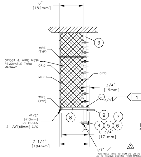
DETAIL A
