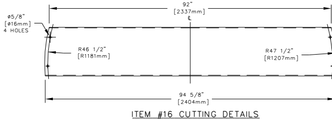
ITEM #16 CUTTING DETAILS 2 REQ'D
