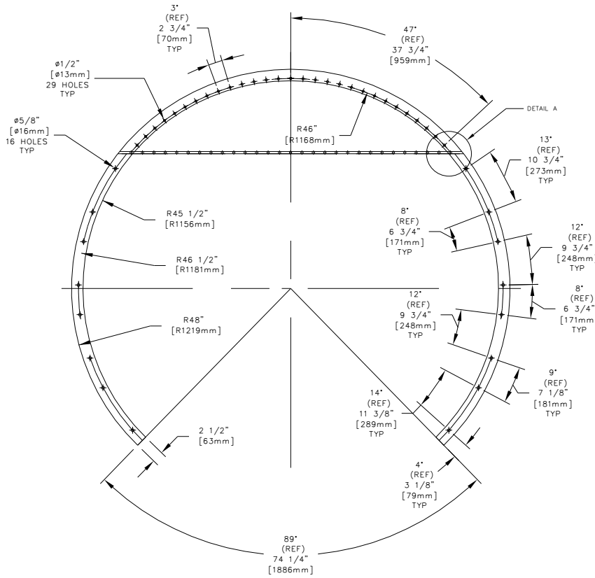
ITEM #3 CUTTING DETAILS 1 REQ'D
