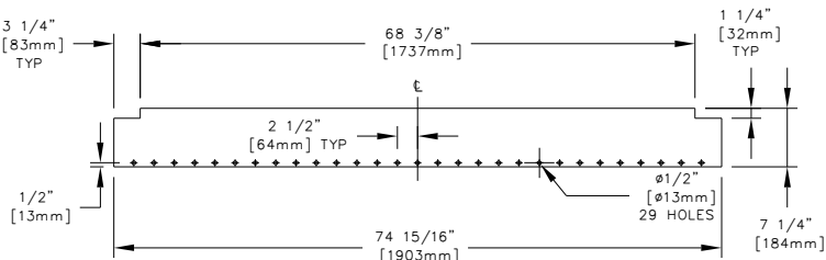
ITEM #8 CUTTING DETAILS 1 REQ'D
