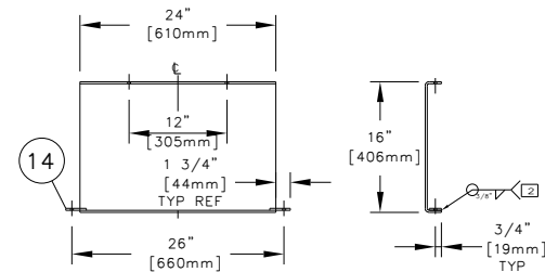
ITEM #13 CUTTING DETAILS 1 REQ'D
