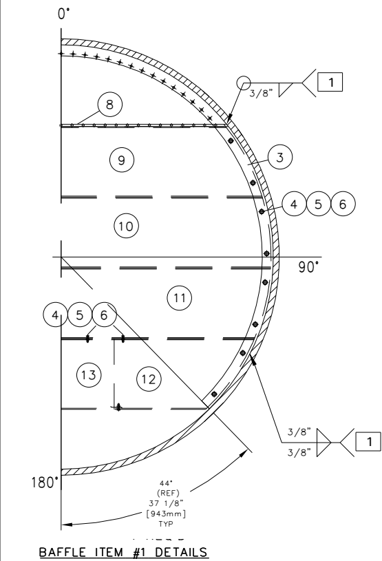
BAFFLE ITEM #1 DETAILS
