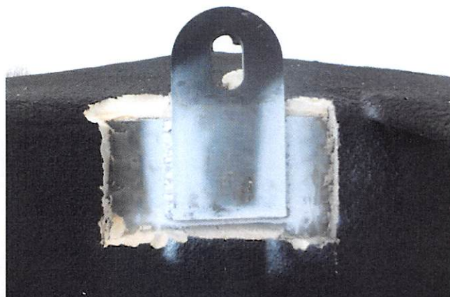
2-lift lugs (typical layout)
