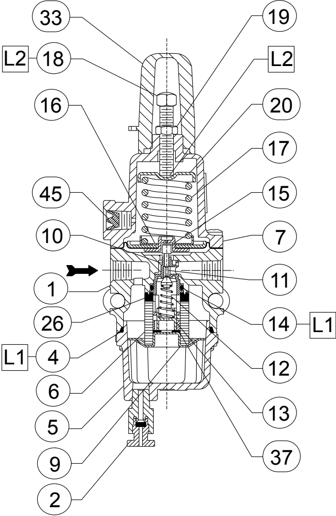
40C1728 APPLY LUBRICANT (L): L1 = MULTI-PURPOSE POLYTETRAFLUOROETHYLENE (PTFE) LUBRICANT L2 = ANTI-SEIZE COMPOUND
