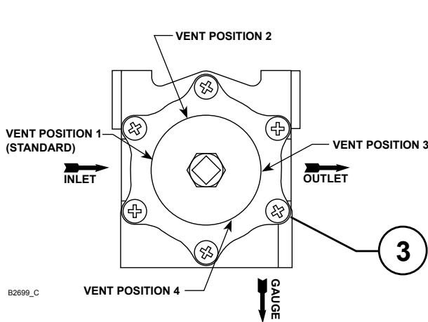
Figure 8. 67C Series Spring Case Vent Positions
