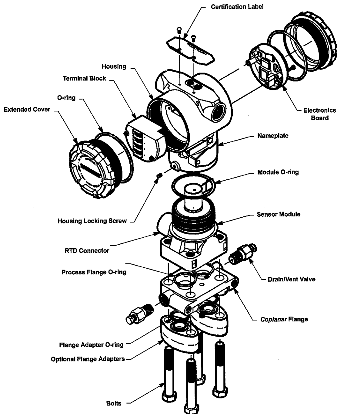
Exploded View of 3095FB Transmitter
