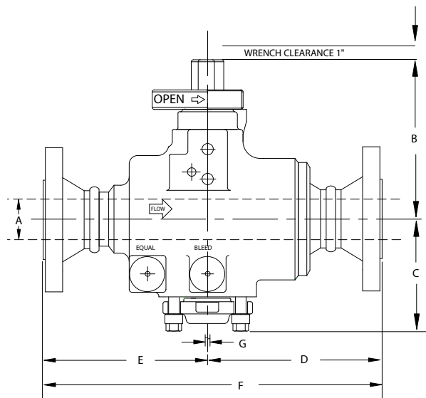
FLANGED TYPE
